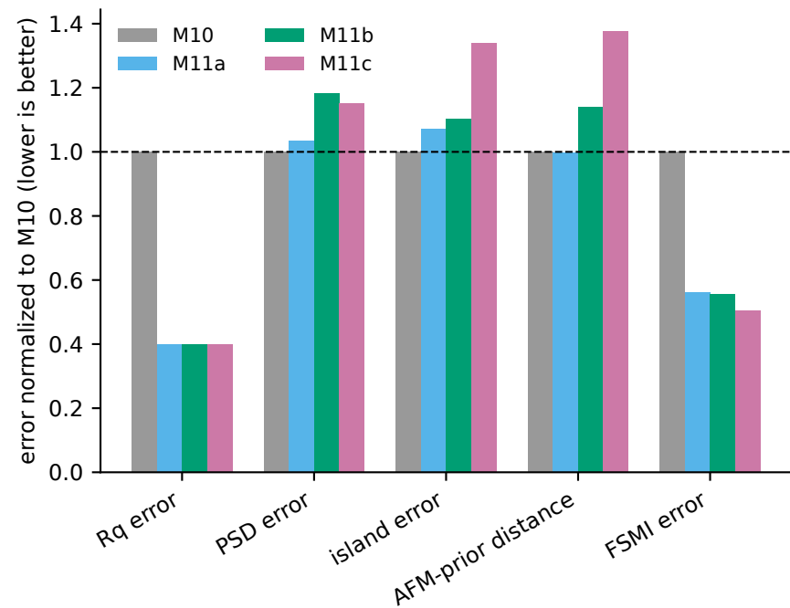
Renderer and conditioning ablation
