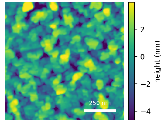
measured AFM Rq=3.09 nm, FSMI=2.92 nm
