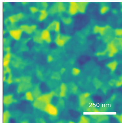
generated AFM Rq=3.64 nm, FSMI=3.27 nm, C=44/100
