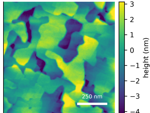
measured AFM Rq=3.23 nm, FSMI=2.66 nm
