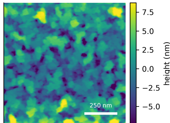
measured AFM Rq=4.34 nm, FSMI=3.81 nm
