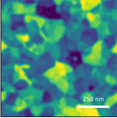
generated AFM Rq=2.24 nm, FSMI=1.77 nm, C=56/100
