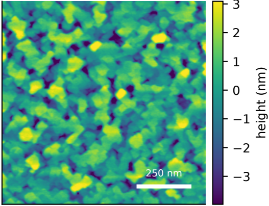
measured AFM Rq=1.86 nm, FSMI=1.57 nm
