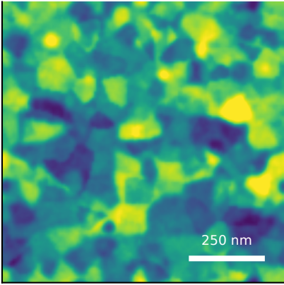
generated AFM Rq=1.97 nm, FSMI=1.95 nm, C=62/100
