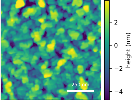
measured AFM Rq=2.46 nm, FSMI=1.97 nm
