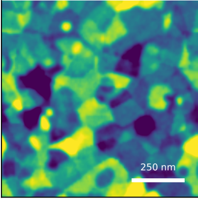
generated AFM Rq=2.96 nm, FSMI=2.71 nm, C=94/100
