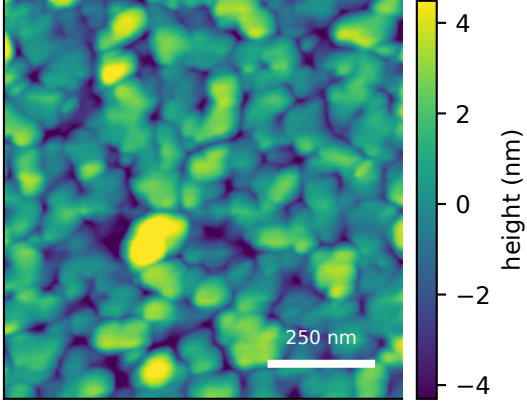
measured AFM Rq=1.96 nm, FSMI=1.60 nm
