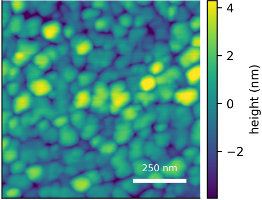
measured AFM Rq=2.06 nm, FSMI=1.71 nm
