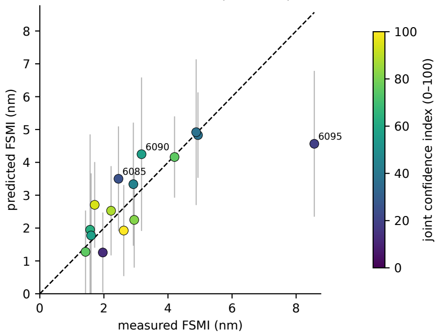
FSMI (nm): Pearson r=0.76 , Spearman \rho=0.83
