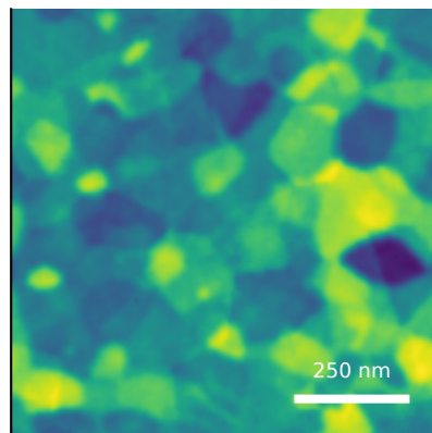
generated AFM Rq=5.79 nm, FSMI=4.57 nm, C=19/100
