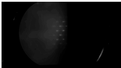
6085 RHEED key frame
