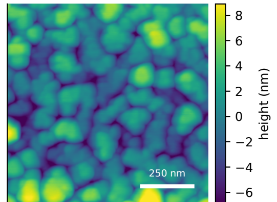
measured AFM Rq=3.13 nm, FSMI=2.46 nm
