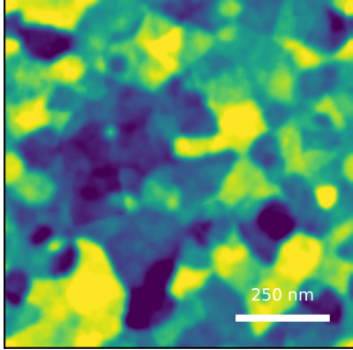
generated AFM Rq=4.03 nm, FSMI=3.75 nm, C=21/100
