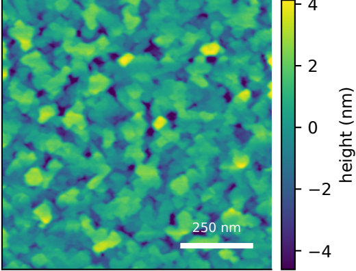
measured AFM Rq=1.65 nm, FSMI=1.28 nm
