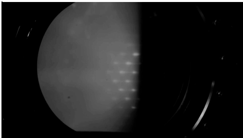
6082 RHEED key frame
