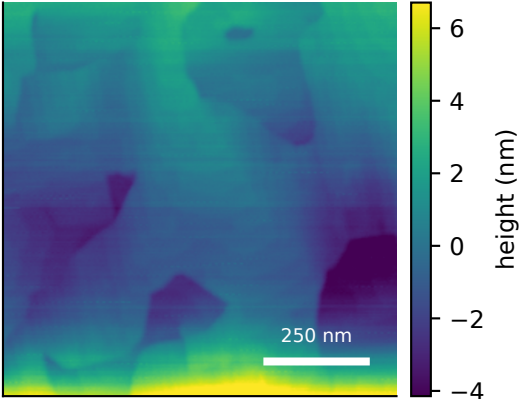
measured AFM Rq=1.47 nm, FSMI=1.43 nm
