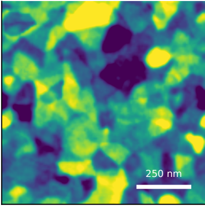
generated AFM Rq=4.53 nm, FSMI=3.65 nm, C=54/100
