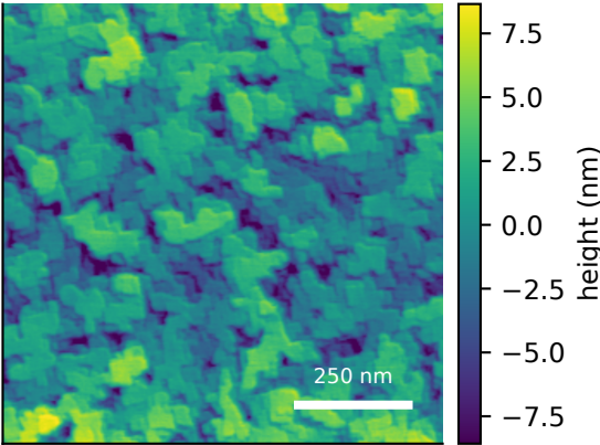
measured AFM Rq=3.05 nm, FSMI=2.62 nm
