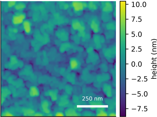
measured AFM Rq=2.56 nm, FSMI=2.22 nm
