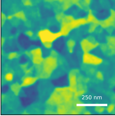
generated AFM Rq=5.28 nm, FSMI=4.71 nm, C=12/100
