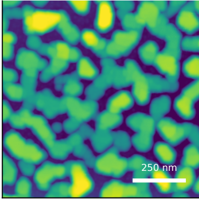
measured AFM Rq=10.32 nm, FSML=9.32 nm
