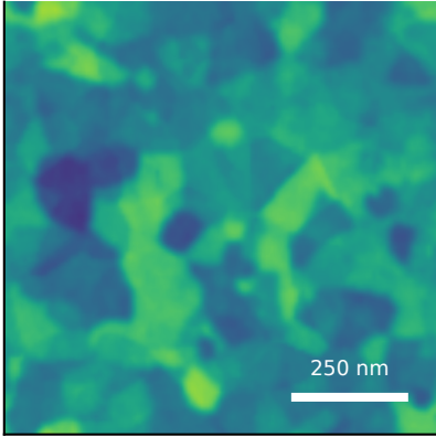
generated AFM Rq=3.68 nm, FSML=3.11 nm, C=21/100
