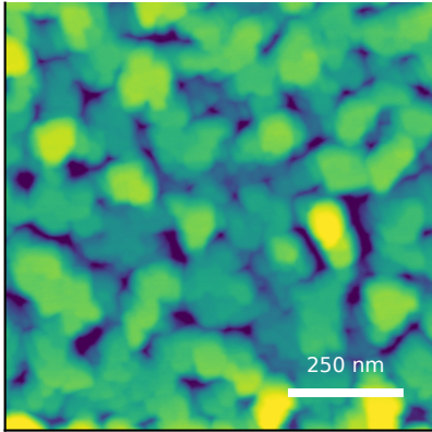
measured AFM Rq=9.87 nm, FSML=8.57 nm
