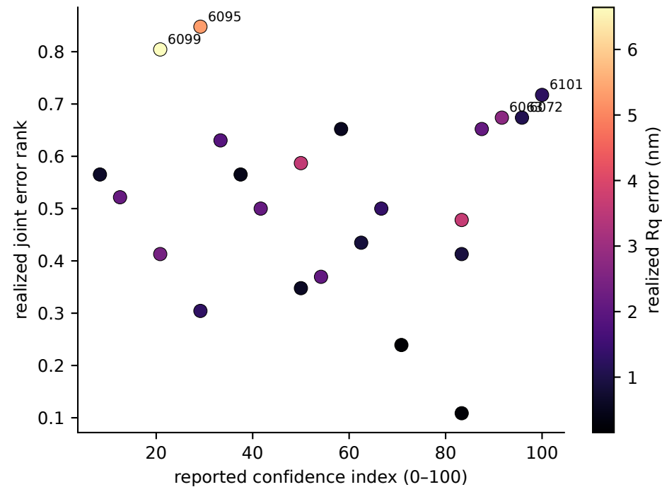
Ranking is not validated: Spearman \rho=0.04 , p=0.85
