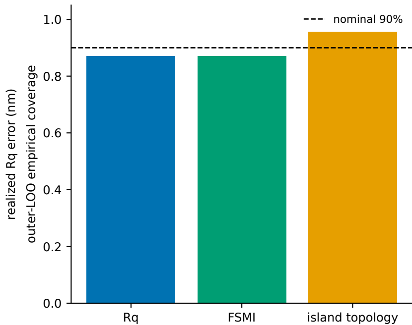
Intervals cover reasonably; pointwise confidence ordering does not
