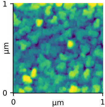
Measured AFM Rq=3.18 nm
