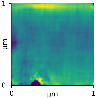
Generated CVAE Rq=3.81 nm
