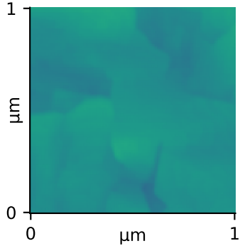
Measured AFM Rq=1.42 nm
