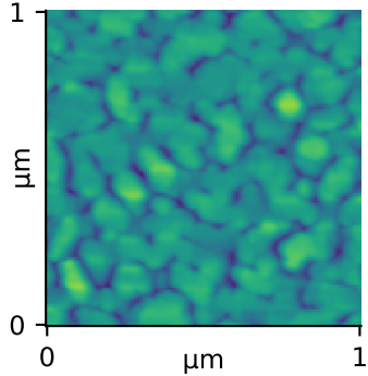
Measured AFM Rq=10.32 nm
