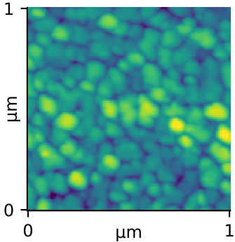
Retrieval (6085) Rq=3.13 nm
