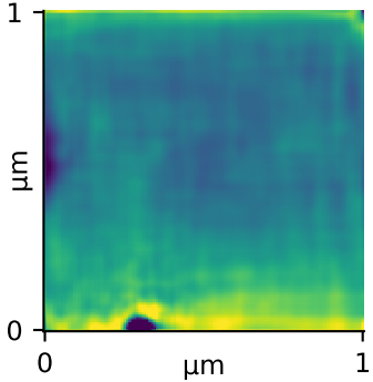
Generated CVAE Rq=3.63 nm
