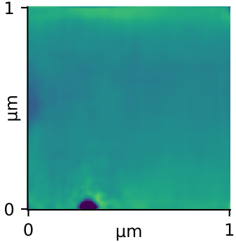
Generated CVAE Rq=3.56 nm
