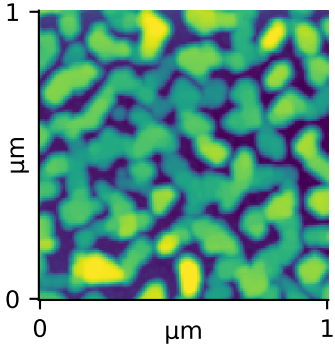
Retrieval (6095) Rq=9.87 nm
