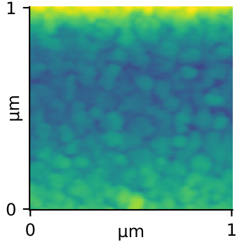
Measured AFM Rq=4.09 nm
