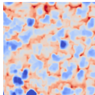
height residual (nm) Rq error=0.82 nm
