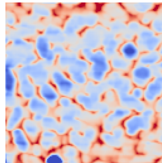
height residual (nm) Rq error=0.46 nm
