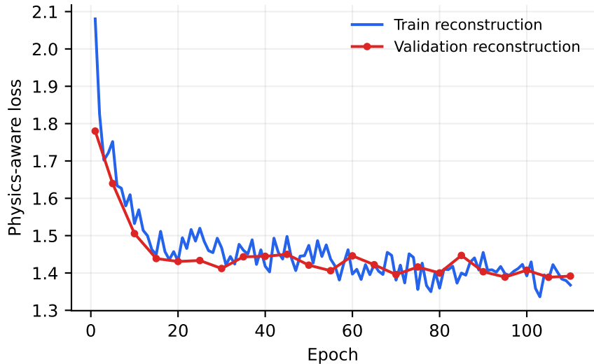
CVAE optimization
