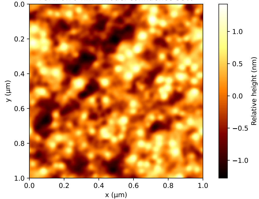
Generated AFM · Sq 0.48 nm FSMI 0.79 nm · model confidence 55%
