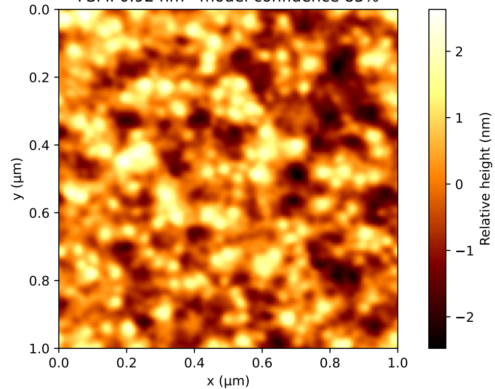
Generated AFM · Sq 0.90 nm FSMI 0.92 nm · model confidence 83%
