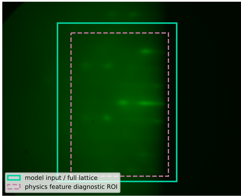
RHEED keyframe 1669 input quality 0.87
