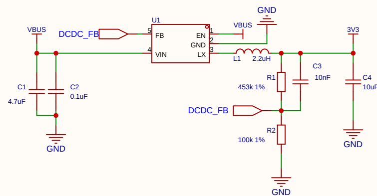
DC-DC USB_5v转3.3v
