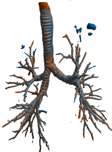
No consistency
