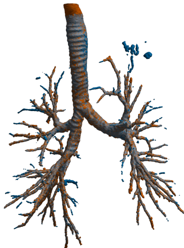
Soft-clDice
