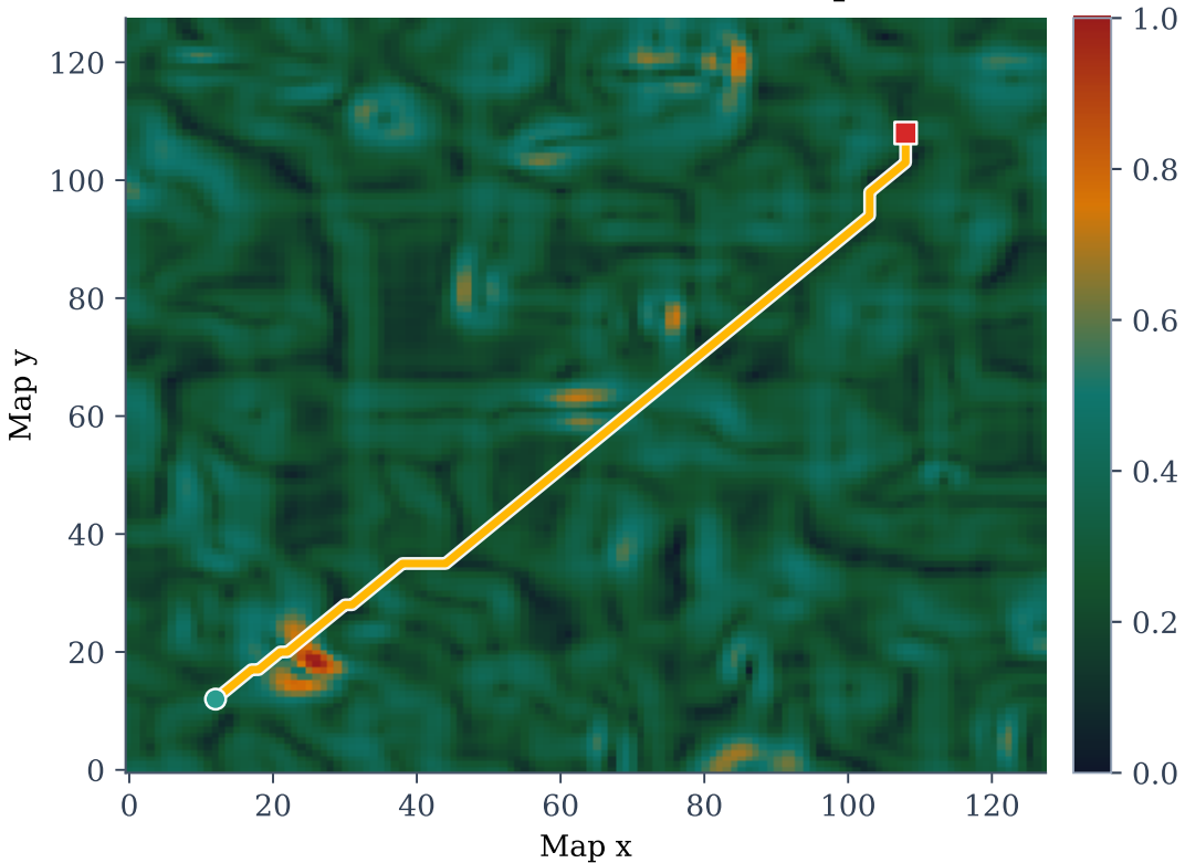
Risk-aware A* over cost map
