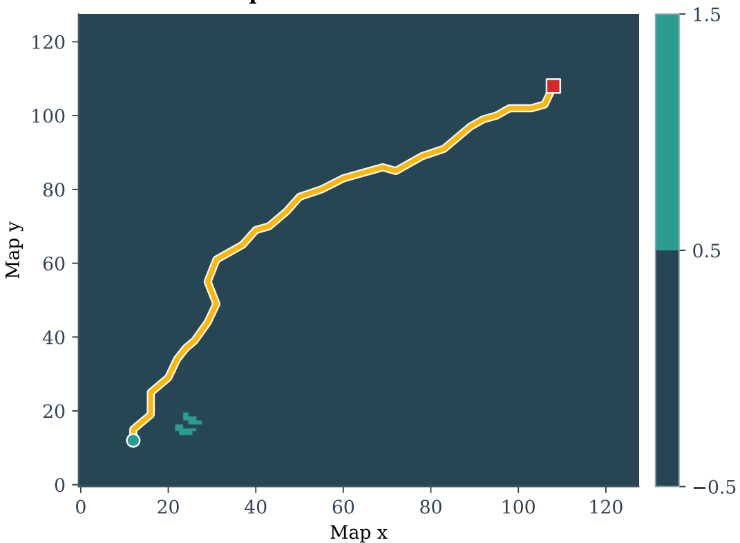
RRT* path over obstacle mask
