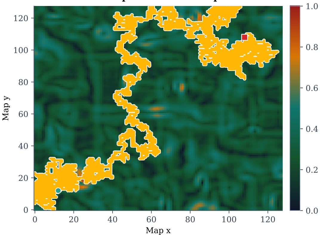
ACO path over cost map
