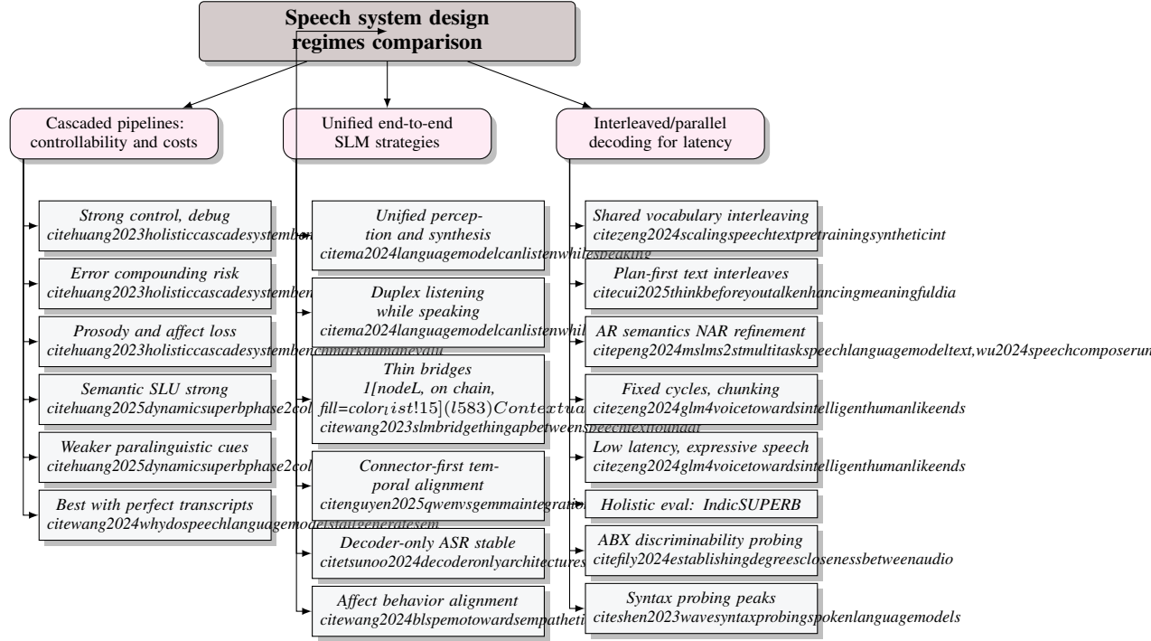
Figure 8: Figure: Cascaded, end-to-end, and interleaved speech systems. The tree contrasts three design regimes for spoken dialogue: cascaded ASR→LLM→TTS pipelines emphasizing control but risking error compounding and paralinguistic loss; unified end-to-end SLMs that reduce hand-offs, enable duplex interaction, and rely on thin projector bridges and targeted alignment (semantic, temporal, affect) to stabilize behavior; and interleaved/parallel decoding that structures when text and speech tokens appear to bound latency while preserving style via AR-on-semantics and NAR refinement. Evaluation guidance highlights multilingual SLU (IndicSUPERB), unsupervised ABX discriminability, and syntax probing to compare semantic vs paralinguistic competence across regimes.
