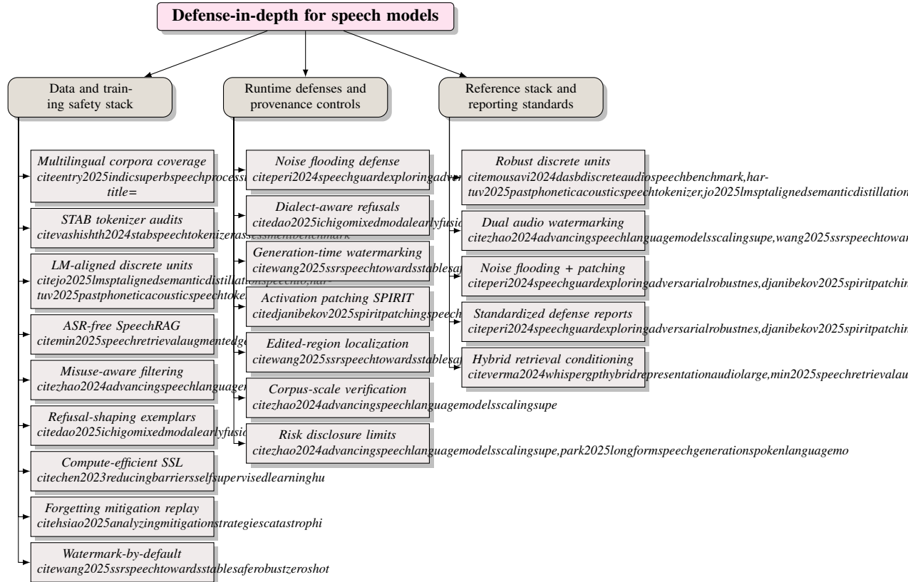
Figure 14: Figure: Defense-in-depth for speech-language systems. The tree organizes safeguards into (1) data and training measures that improve coverage, robustness, and safety alignment; (2) runtime defenses and provenance tools that harden inputs/outputs and enable post-hoc mitigation and verification; and (3) a reference stack with recommended components and reporting standards. Arrows in the conceptual figure flow from pre-deployment preparation to inference-time protection and auditing, emphasizing layered, complementary controls across the lifecycle.
