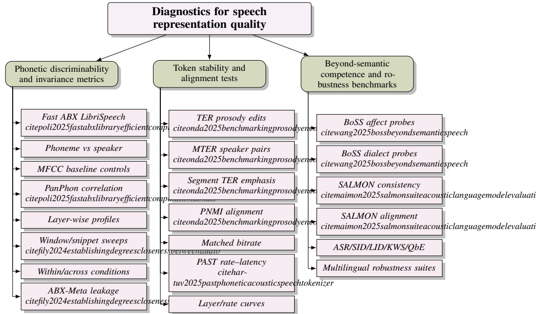
Figure 3: Figure: Hierarchical diagnostics for speech representation quality. The suite organizes (1) phonetic discriminability/invariance via fast ABX with MFCC baselines, PanPhon correlations, layer-wise profiles, and snippet sweeps to expose leakage across factors; (2) decoder-free token stability and linguistic alignment using TER/MTER under controlled WORLD prosody edits, segment-restricted TER for emphasis, PNMI, and PAST operating points to select layer/rate–latency–fidelity trade-offs; and (3) beyond-semantic competence and robustness through BoSS affect/dialect probes and SALMON consistency/alignment tasks, extensible to broader multilingual ASR/SID/LID/KWS/QbE coverage.
