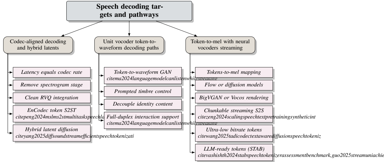
Figure 4: Figure: Decoding targets and pathways. The tree groups practical speech decoding routes into three categories: codec-aligned decoding (including hybrid token-conditioned latents) for minimal conversion loss and codec-rate latency; unit vocoder token-to-waveform paths that preserve modularity and enable promptable style control and full-duplex behavior; and token-to-mel pipelines that map tokens to mel spectrograms, leveraging flow/diffusion and mature neural vocoders for chunkable, streaming-friendly synthesis. The LLM-ready token interface vetted by STAB facilitates controllable streaming and policy-aware scheduling, exemplified by StreamUni.
