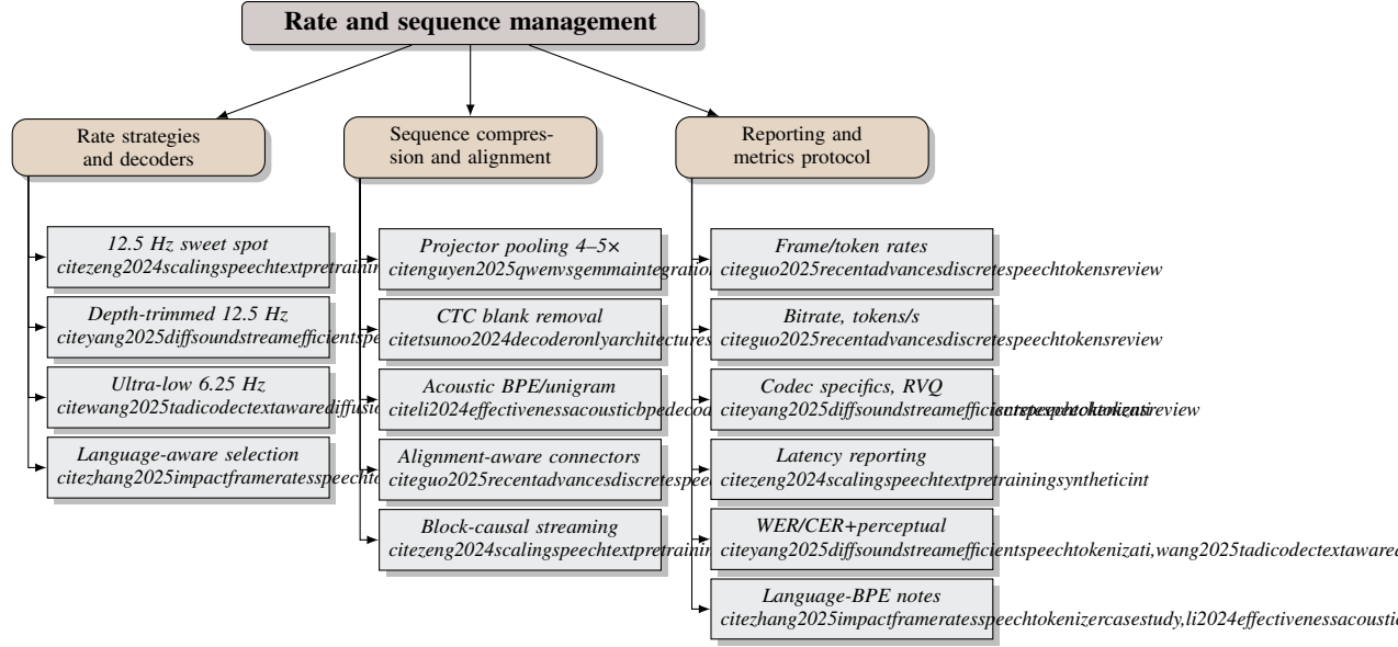
Figure 2: Figure: Hierarchical overview of rate and sequence management. Left: strategy space balancing frame rates and decoder strength (12.5 Hz sweet spot, depth-trimmed hybrids, and ultra-low 6.25 Hz with text-aware diffusion). Middle: sequence compression and alignment mechanisms (projector pooling, CTC blank removal, acoustic BPE, alignment-aware connectors, and block-causal streaming). Right: standardized reporting protocol covering rates, bitrate, compression stats, codec specifics, latency, and coupled accuracy–perceptual metrics with language/BPE notes.
