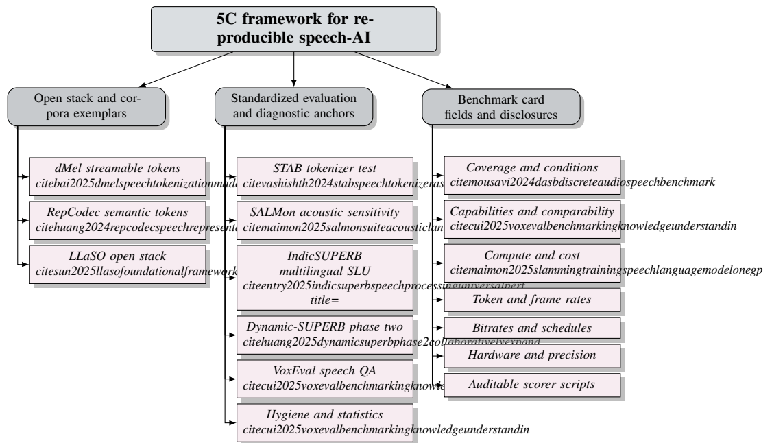
Figure 15: This figure shows a two-level 5C overview for reproducible speech-AI, grouping content into: (1) open stack exemplars (tokenizers/codecs and corpora), (2) standardized evaluation anchors (low-cost, rate-/robustness-aware diagnostics), and (3) benchmark card disclosures (coverage, conditions, comparability, and compute/cost reporting). Together, these pillars link open, inspectable pipelines to comparable cross-lab evaluation via explicit, auditable reporting.
