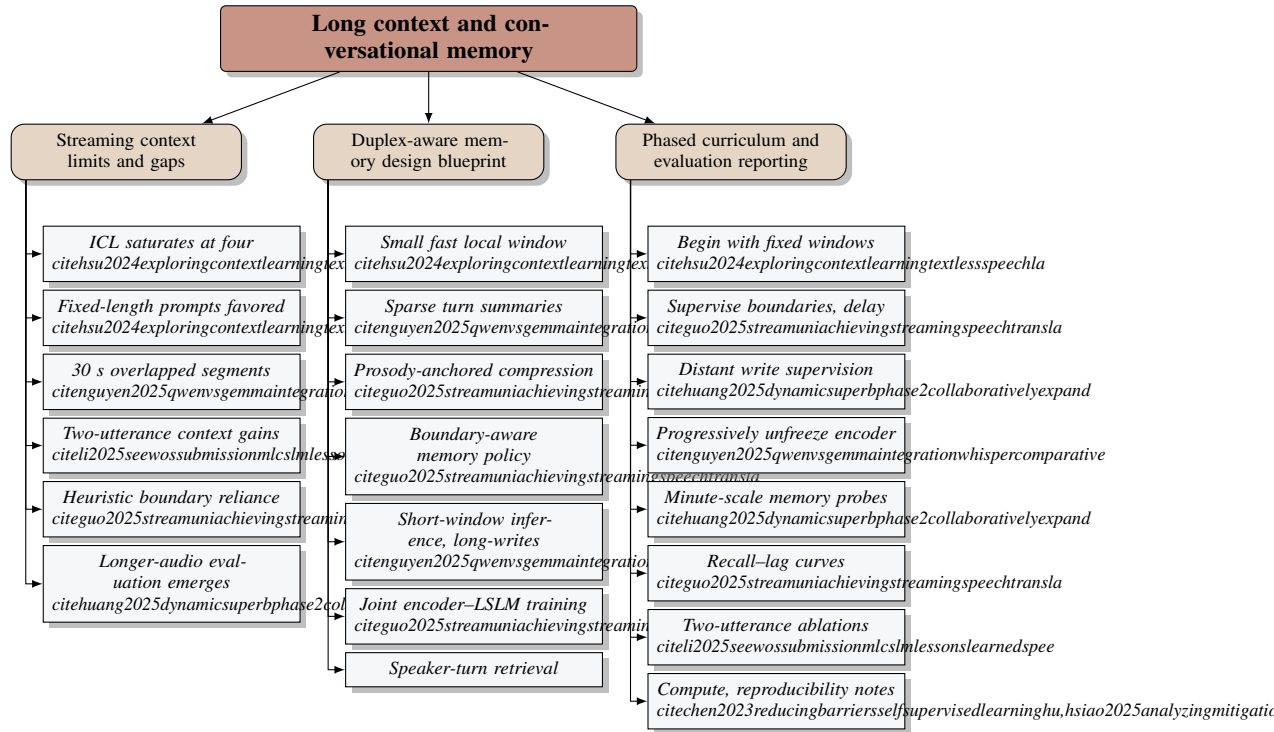
Figure 16: Figure: Duplex-aware long-context memory for streaming speech agents. The chart organizes (1) current streaming limitations (few-shot ICL saturation, segmentation and boundary heuristics), (2) a practical memory blueprint (small local windows plus sparse, turn-synchronous summaries with prosody-aware compression and joint encoder–LSLM policy alignment), and (3) a phased curriculum with evaluation/reporting (fixed-window warmup, boundary/delay supervision, distant supervision, progressive unfreezing, and memory-centric probes/metrics). Together, these components map constraints to design choices and training–evaluation practices for robust, low-latency duplex dialogue.
