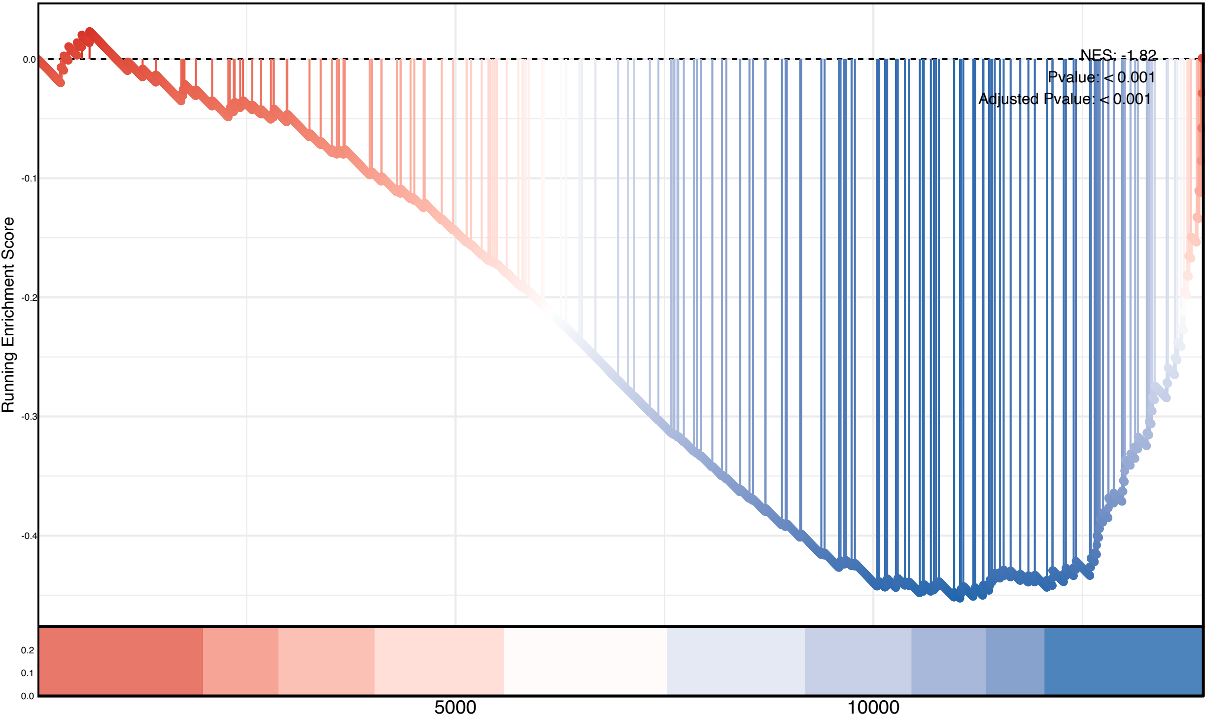
Estrogen Response Early
