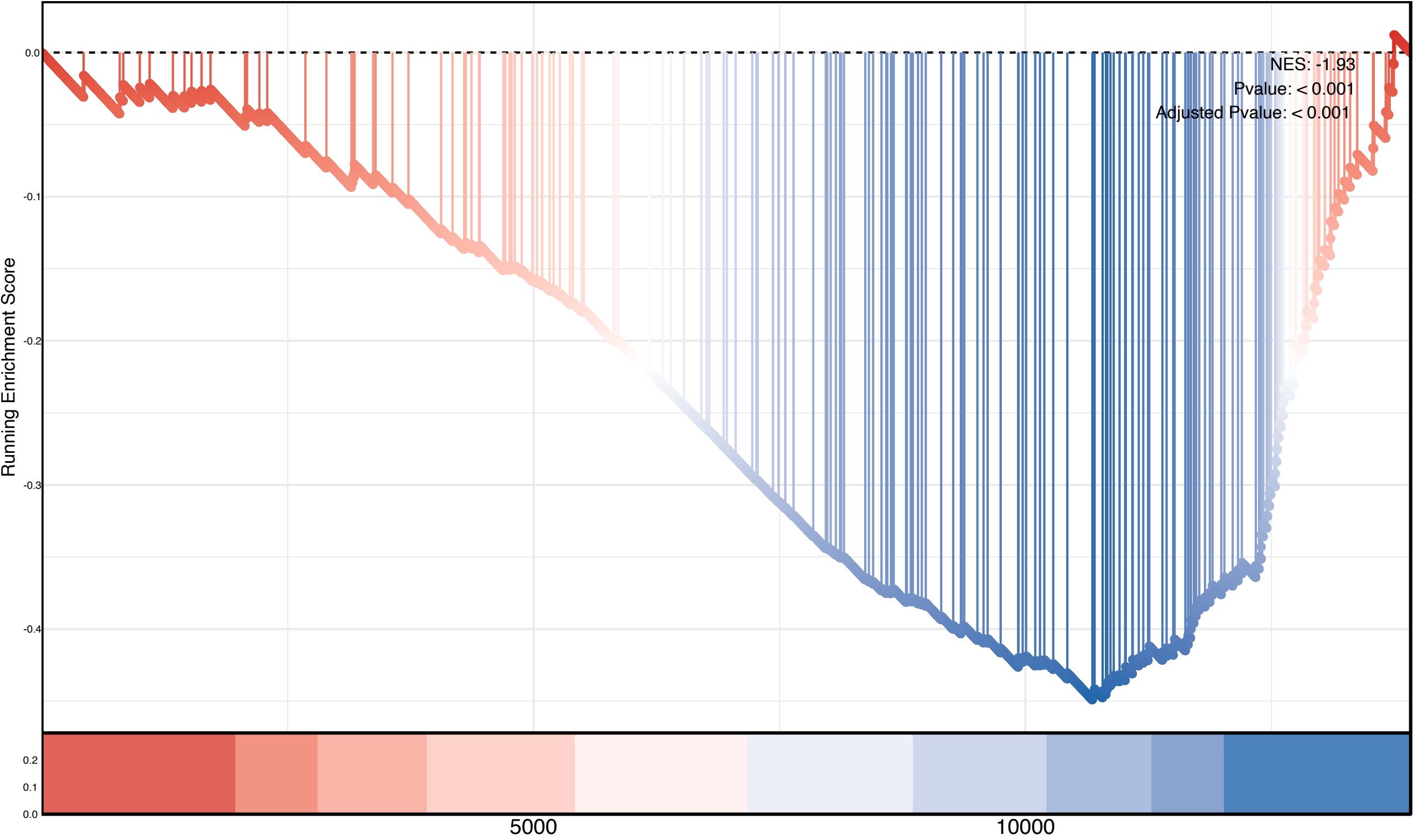
Treg Vs Tconv Cd4 Tcell From Ln Up
