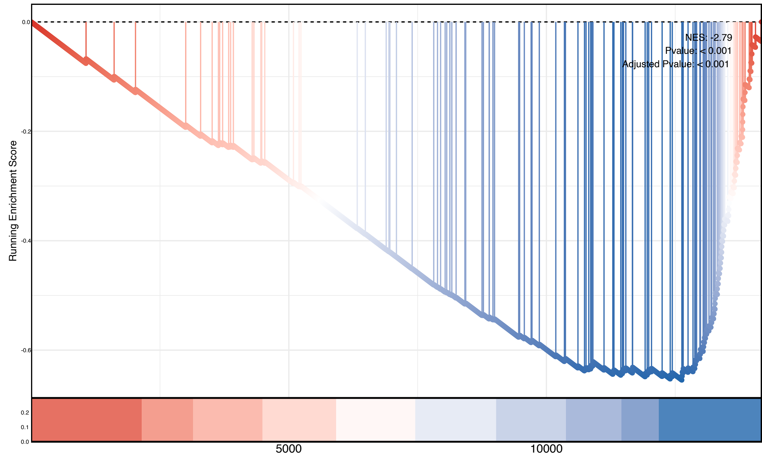
Dna Replication Pre Initiation
