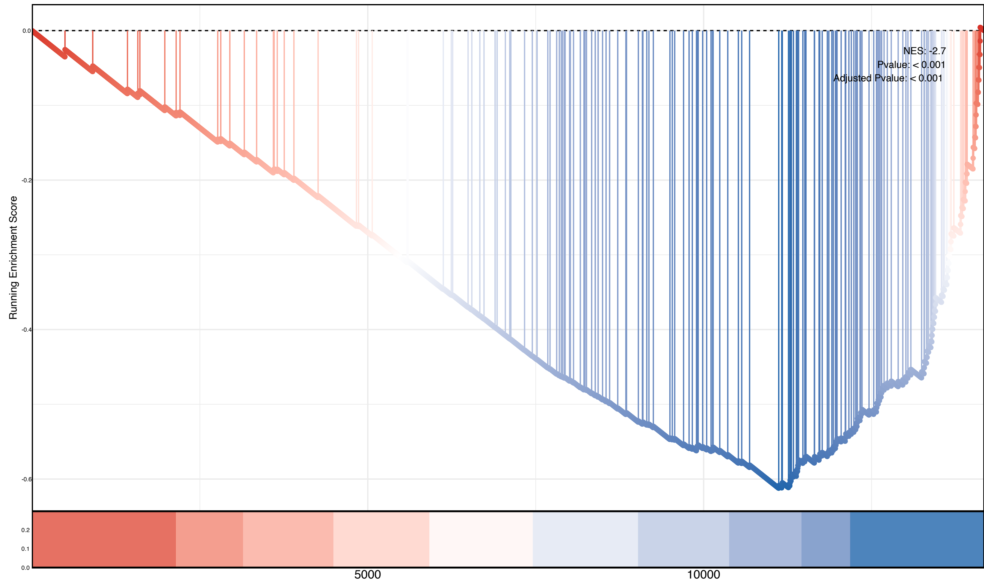
Teff Vs Tconv Day5 In Culture Up
