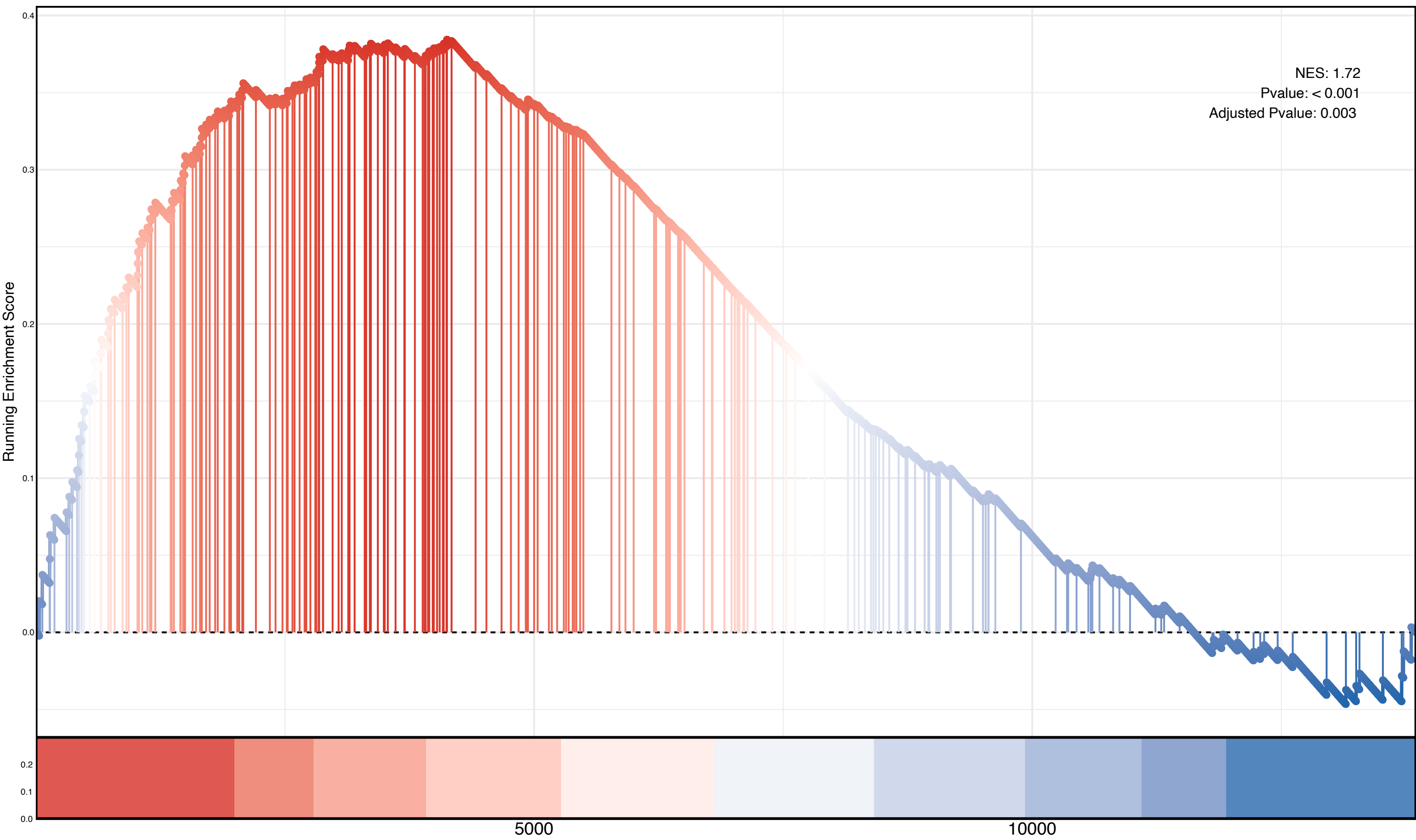
Gtpase Activator Activity
