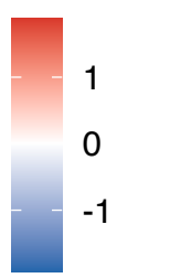
Z-Score
