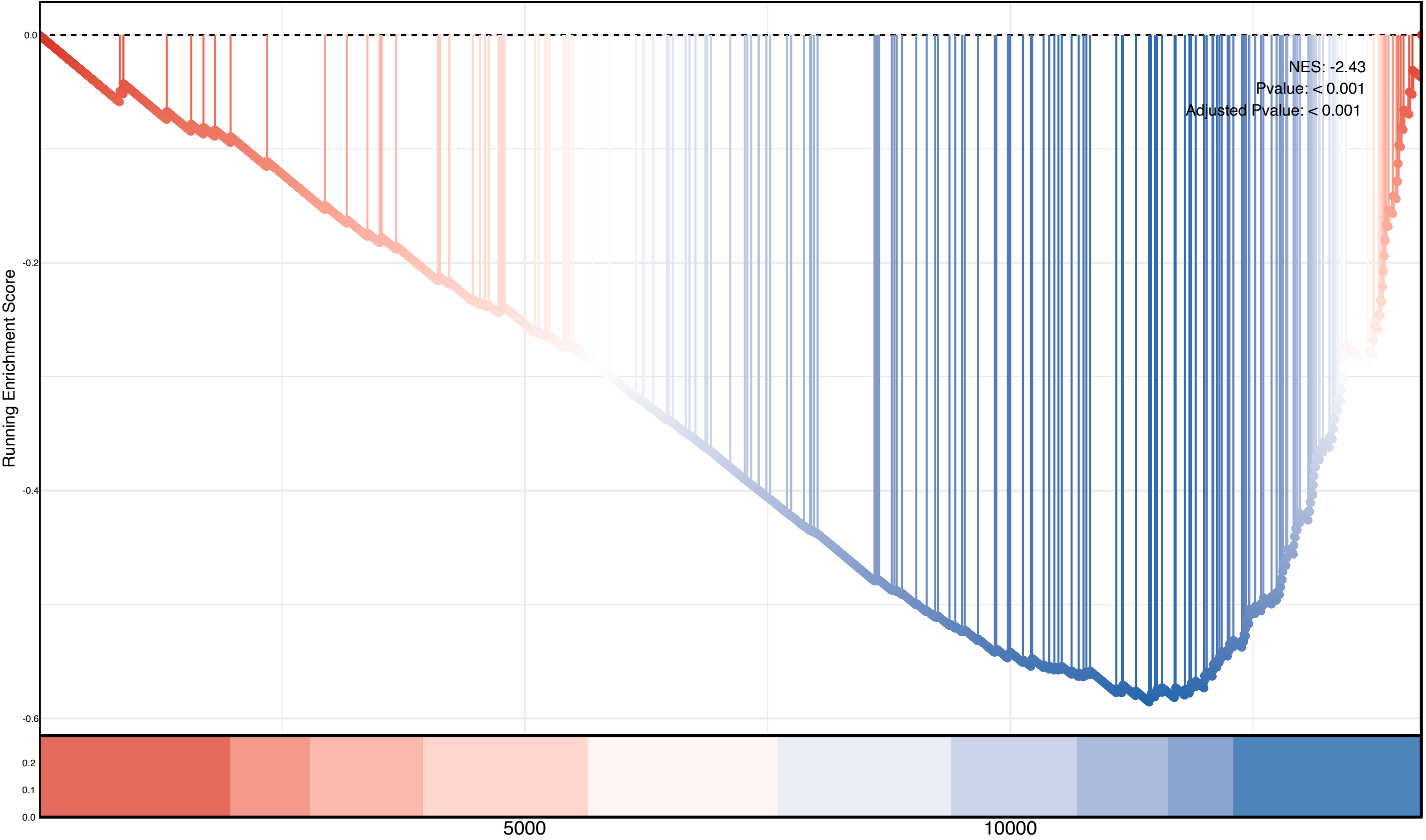
Pdc Vs Tgfb1 Treatedcommon Dc Progenitor Up
