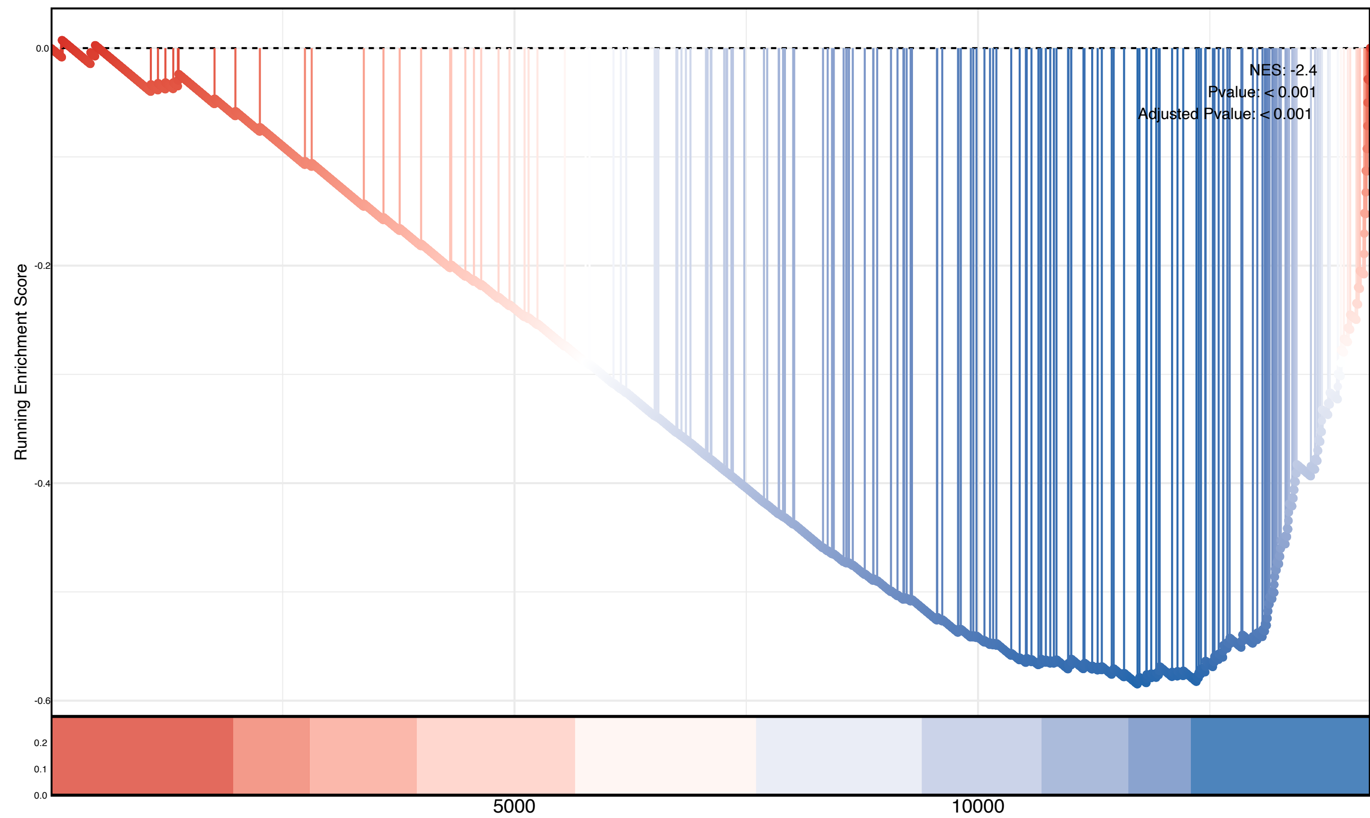
Unstim Vs Stim Memory Tcell Dn
