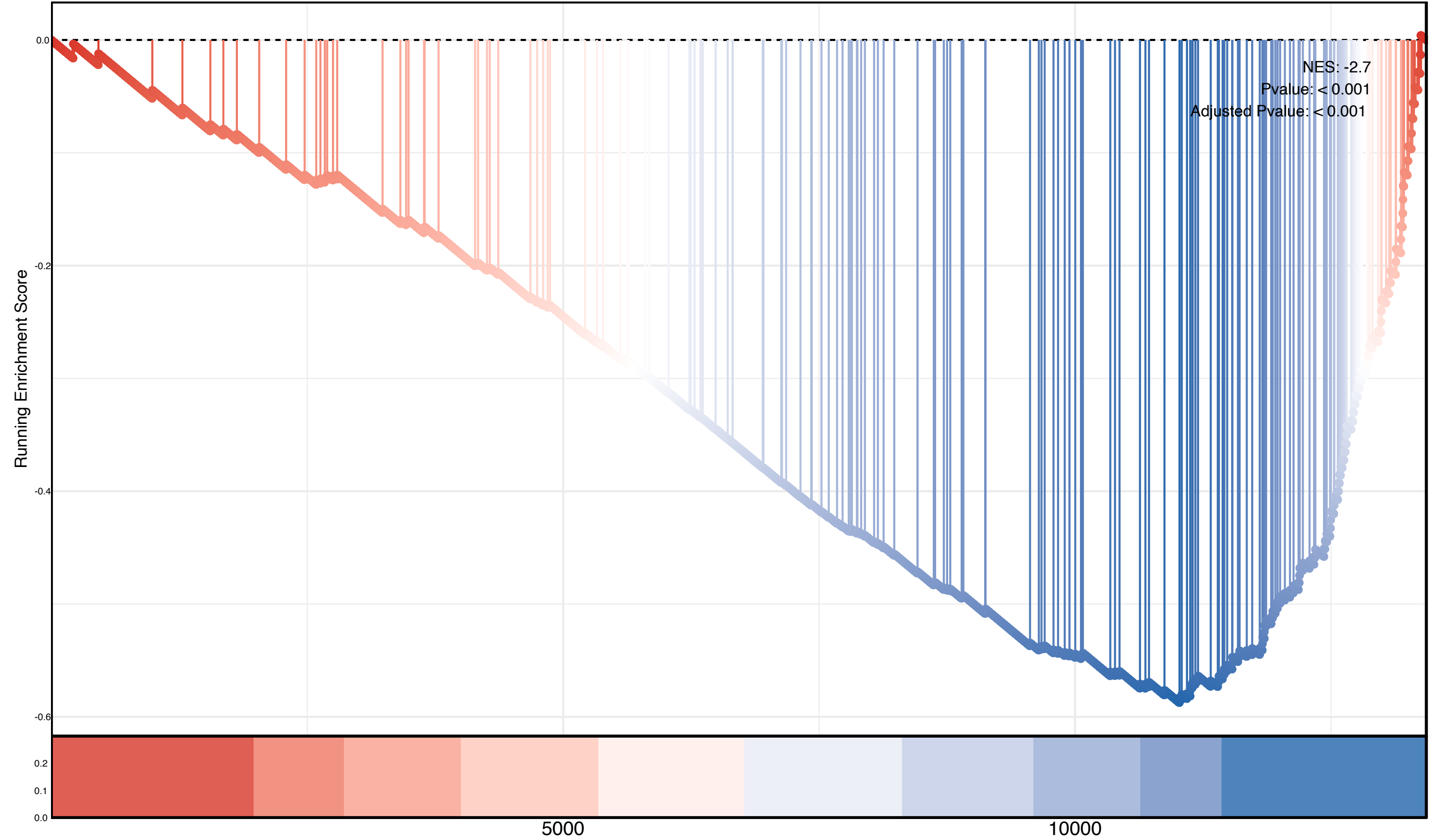
G2m Checkpoint
