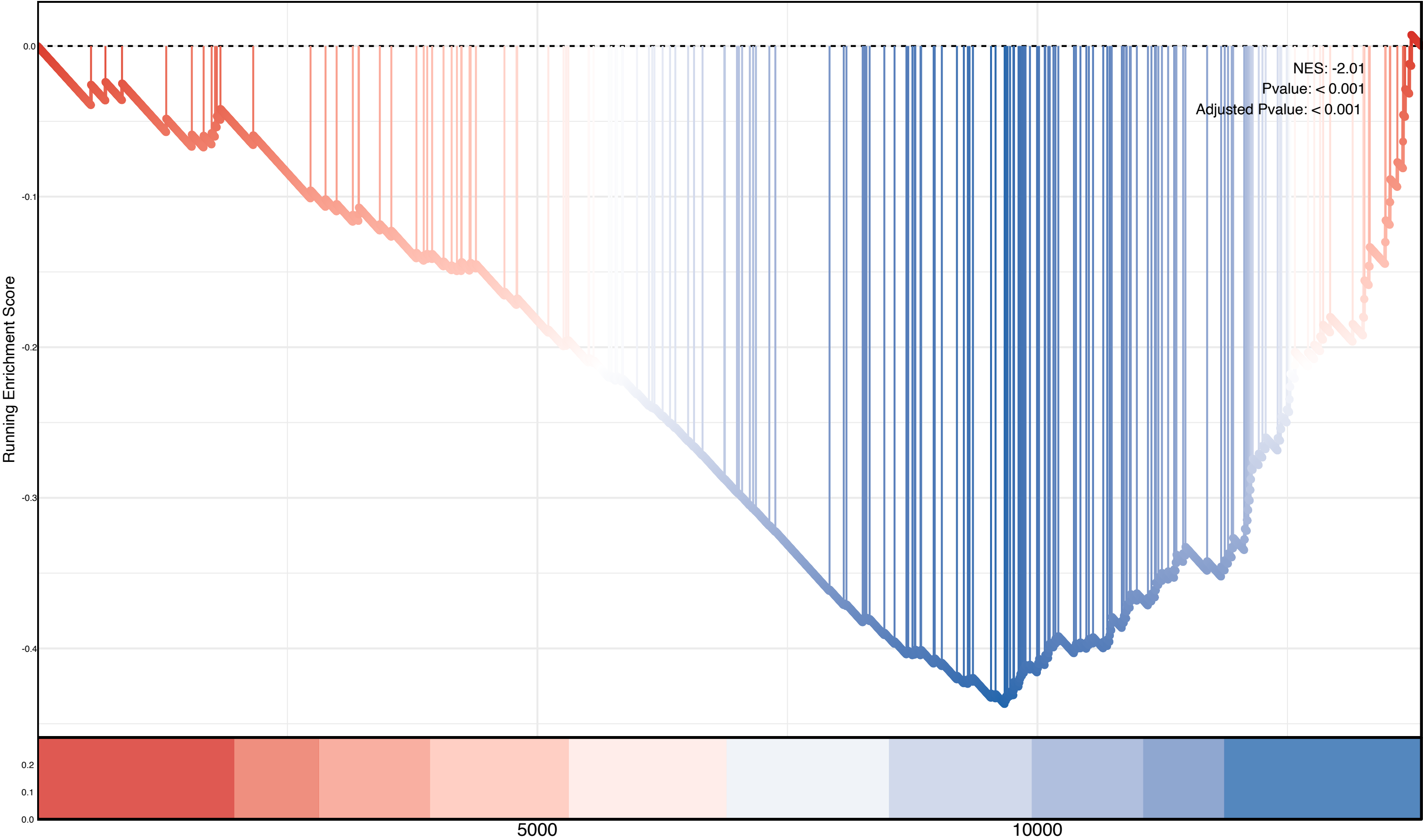
Trna Metabolic Process
