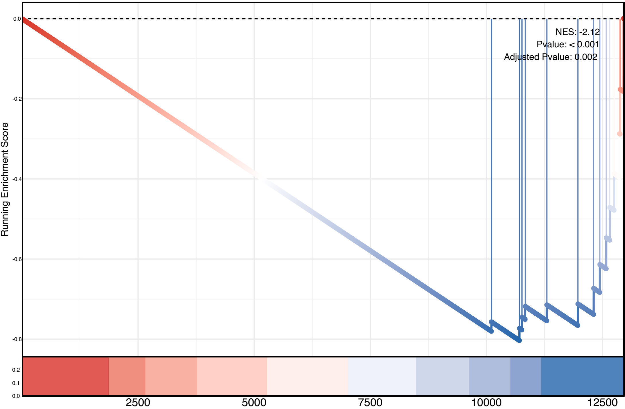
Sm Pathway
