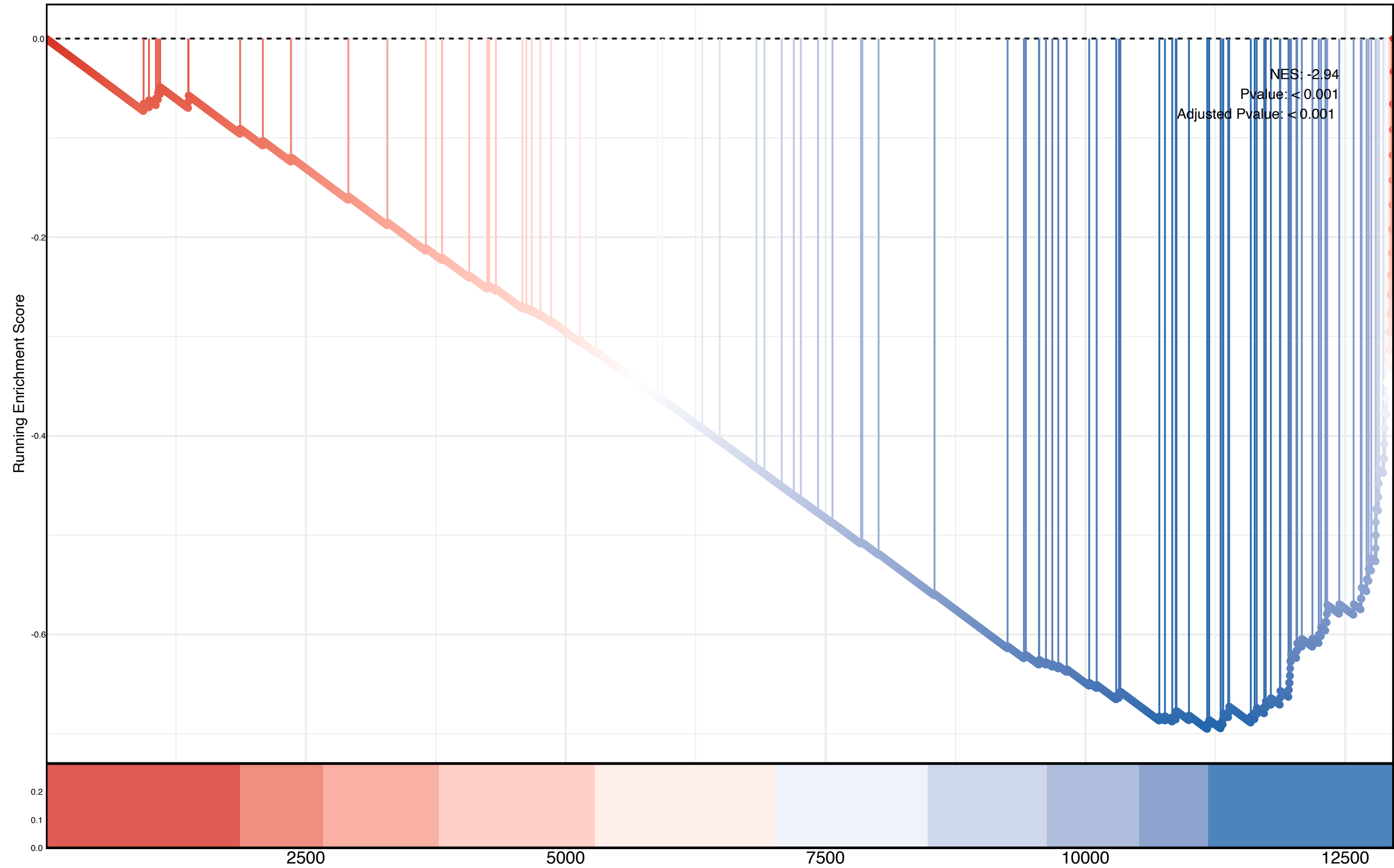
Mrna Polyadenylation
