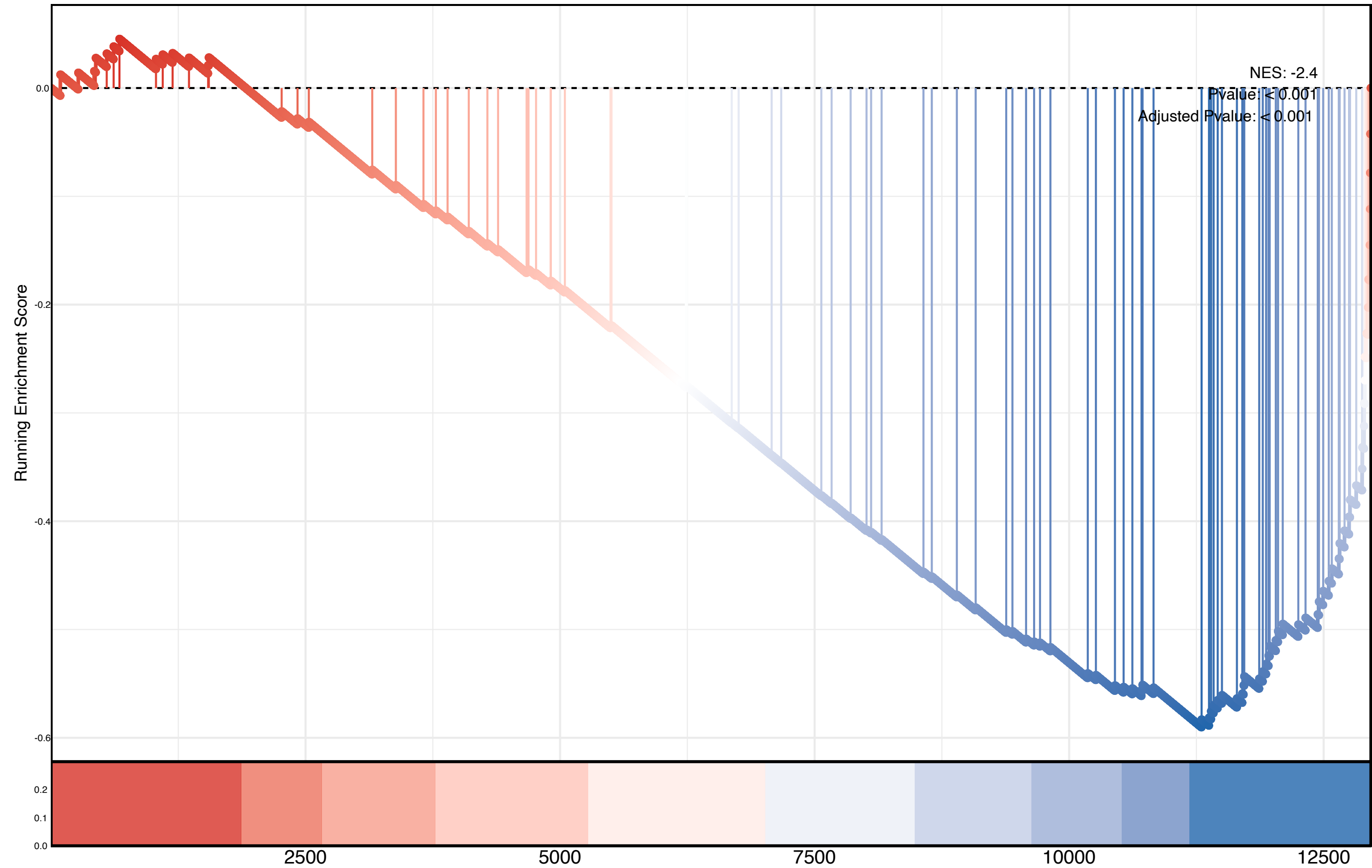
Regulation Of Mrna Splicing Via Spliceosome
