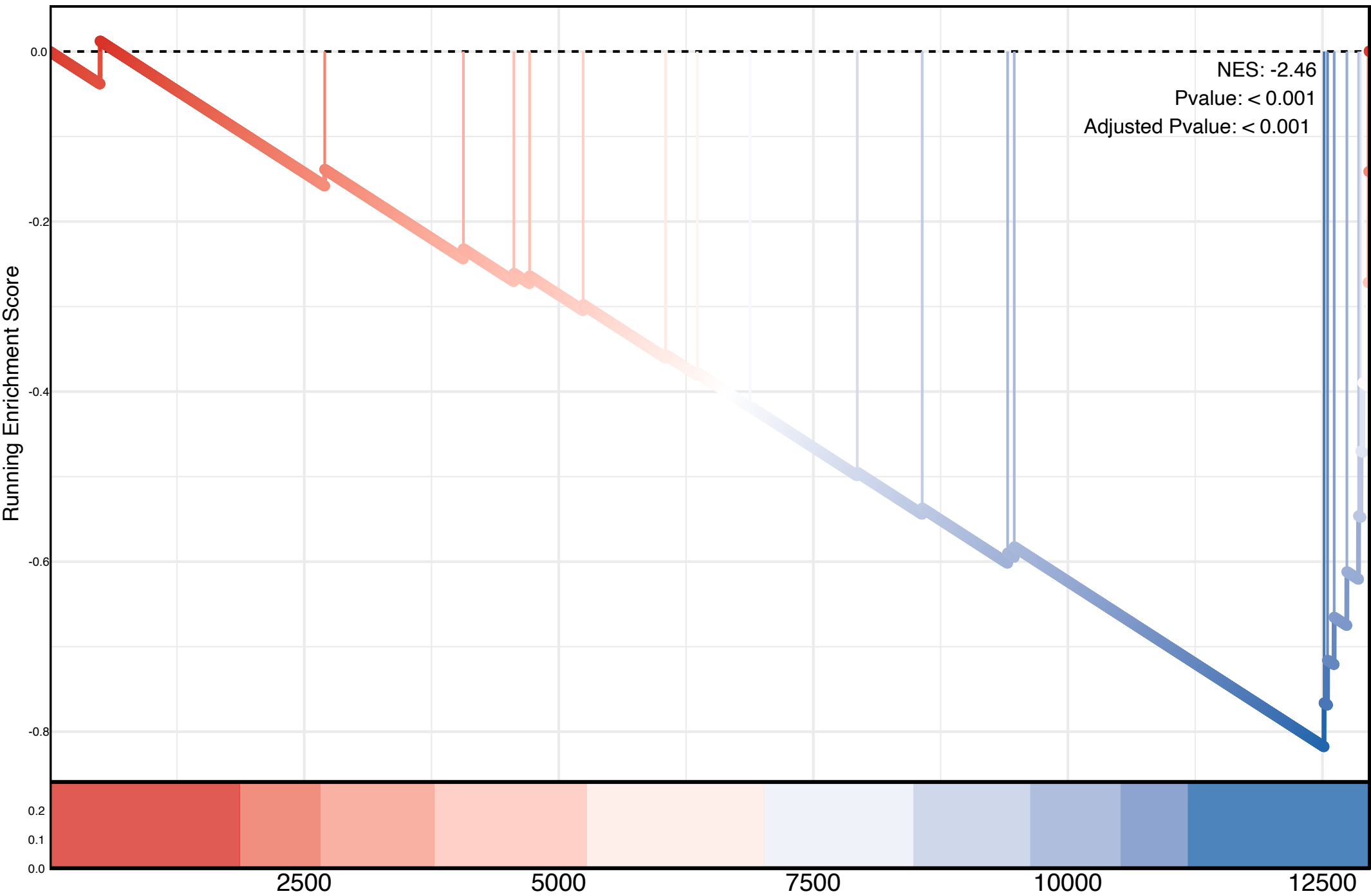
Poly Pyrimidine Tract Binding
