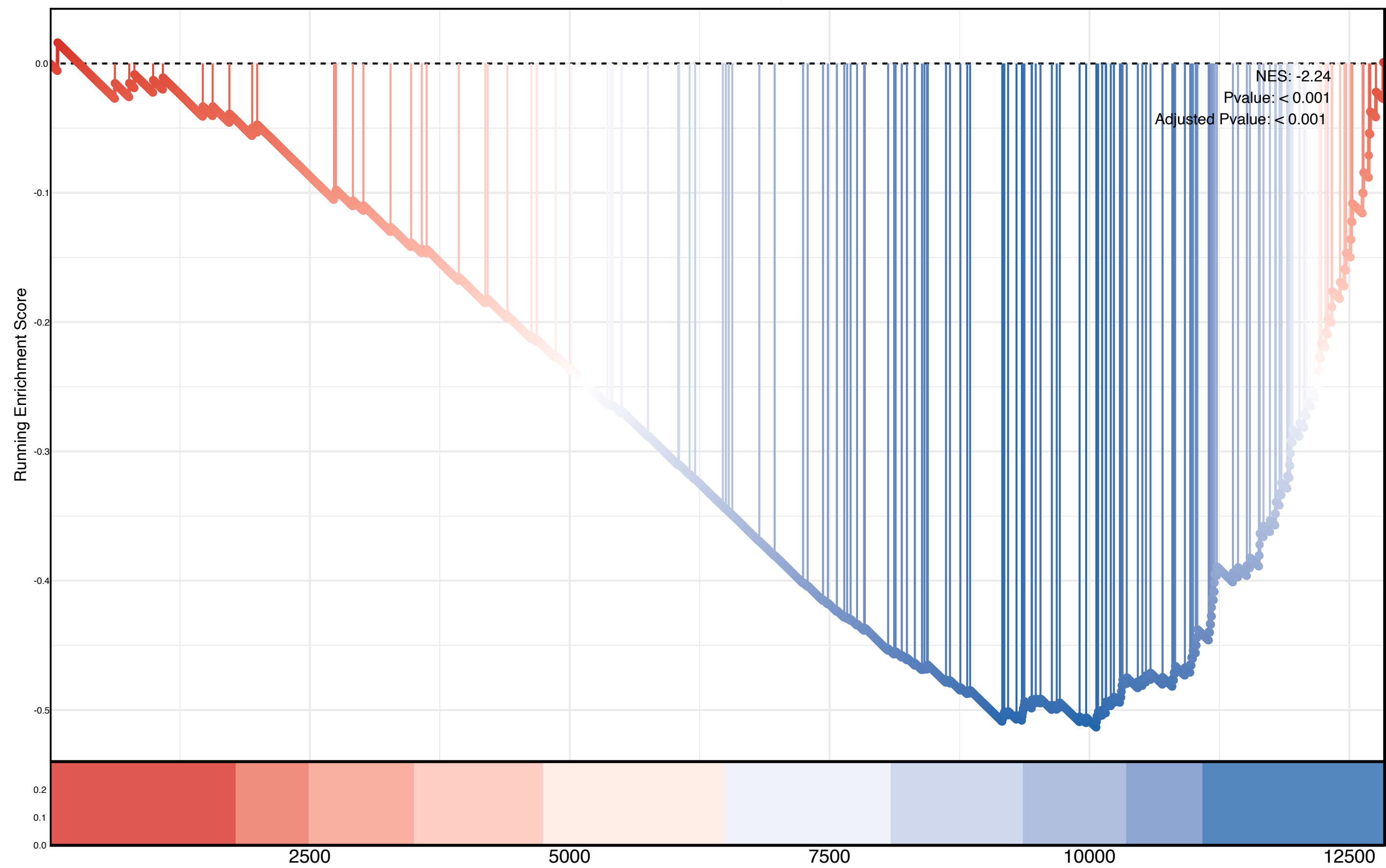
Mitochondrial Gene Expression
