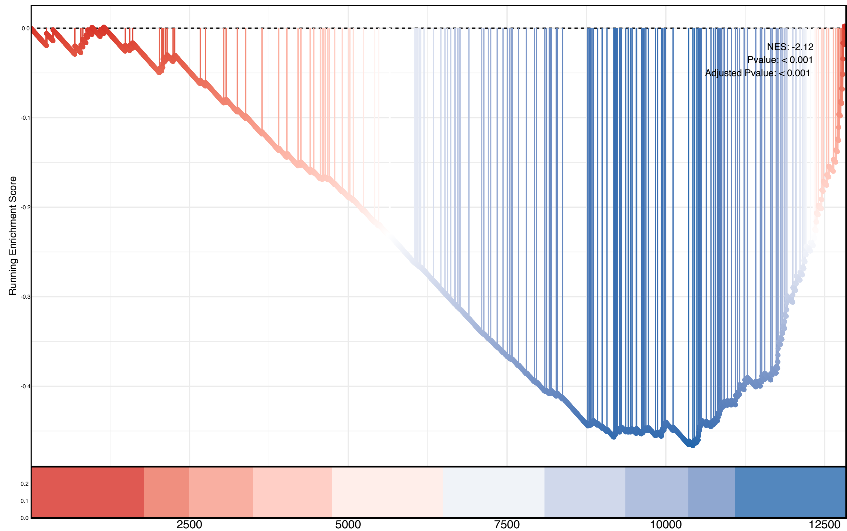
Amino Acid Metabolic Process
