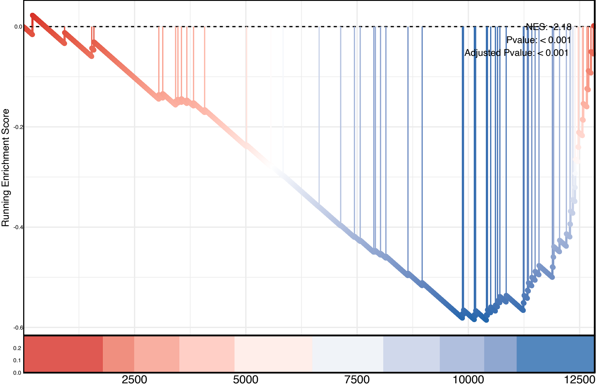
Dna Helicase Activity
