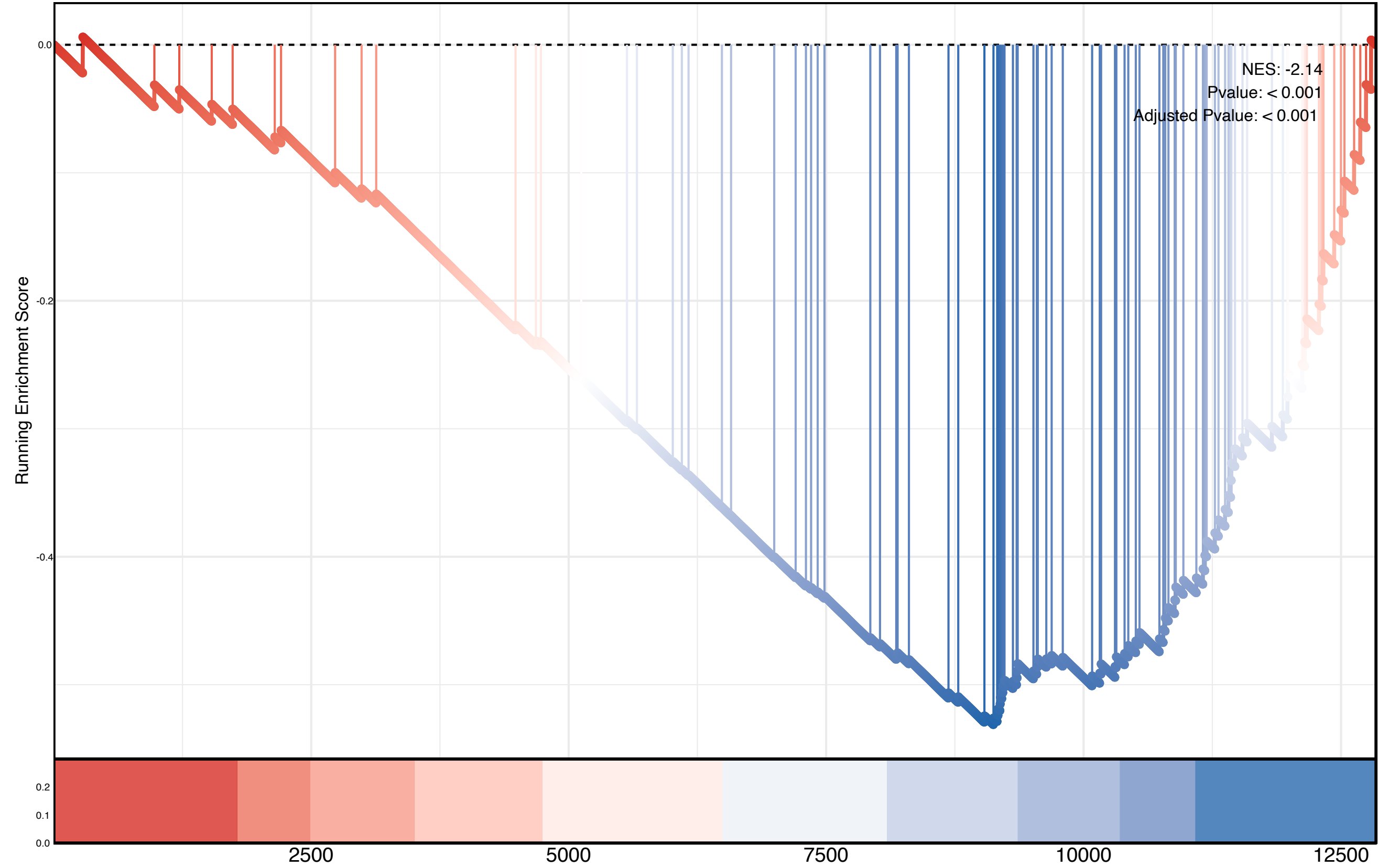
Decreased Activity Of Mitochondrial Complex I
