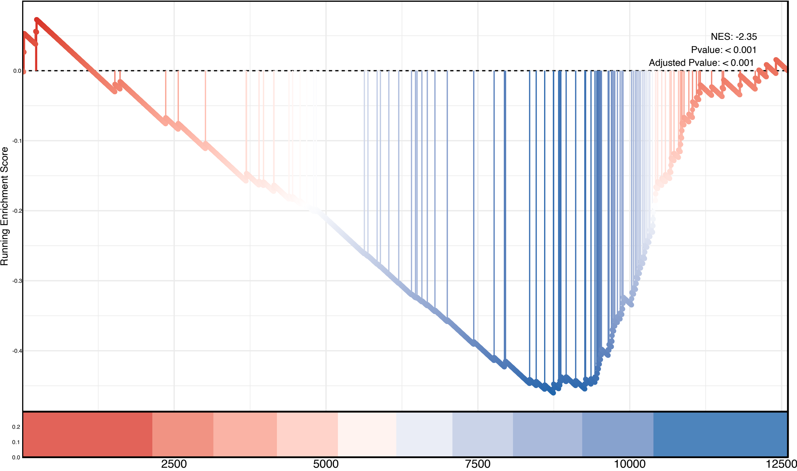
Cell Cycle
