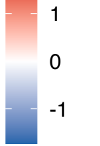
Z-Score
