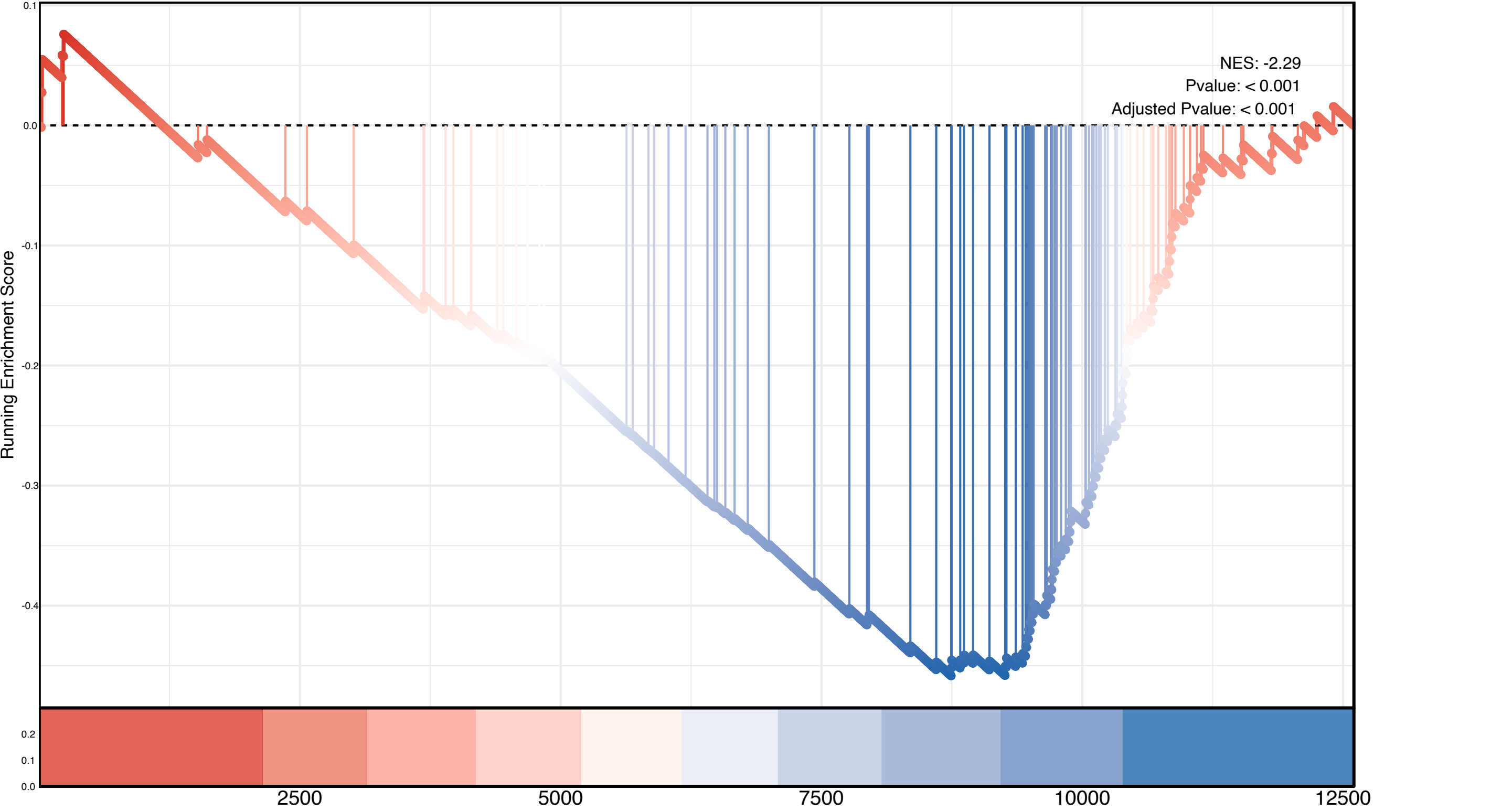
Cell Cycle
