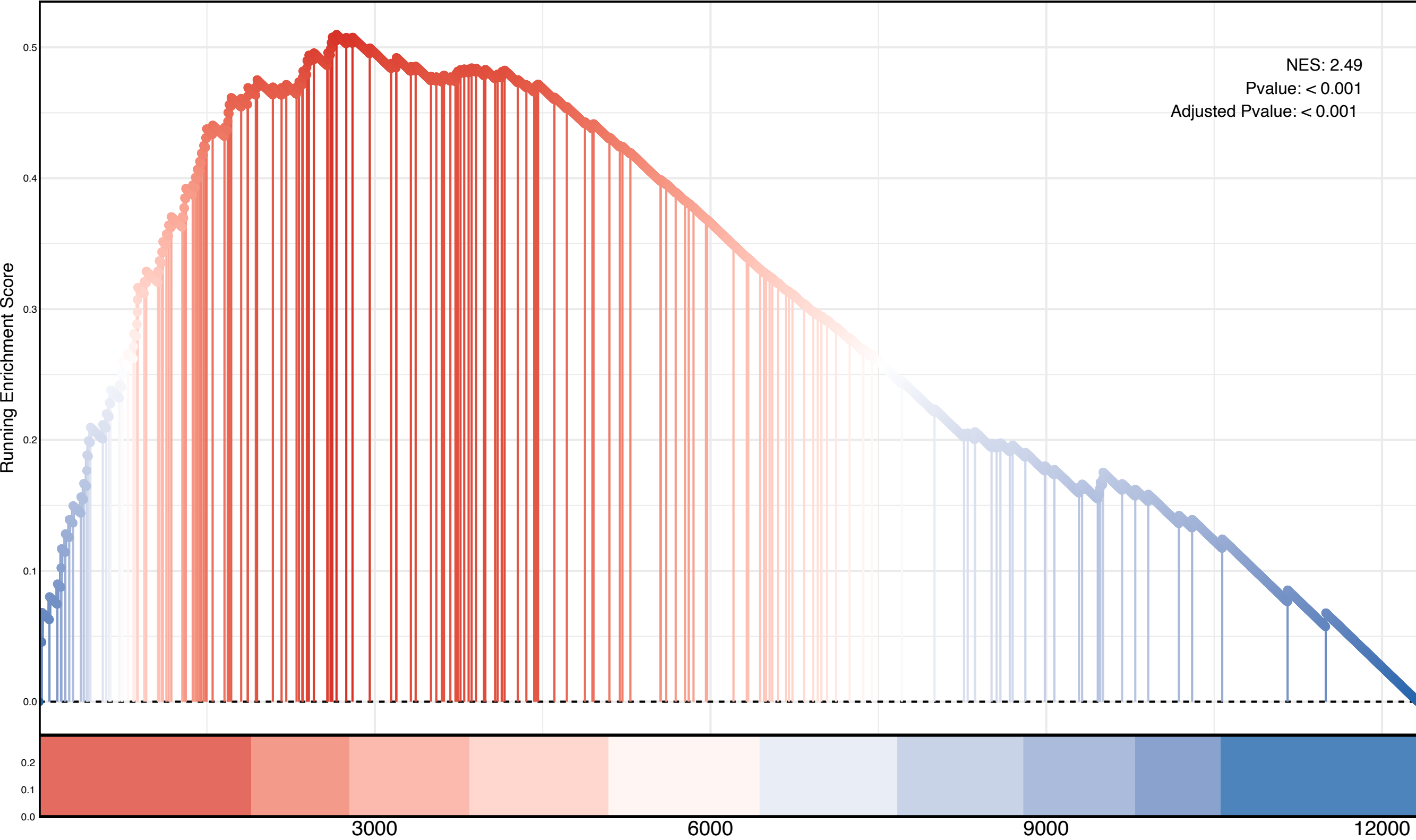
Naive Vs Activated Cd8 Tcell Mir155 Ko Dn
