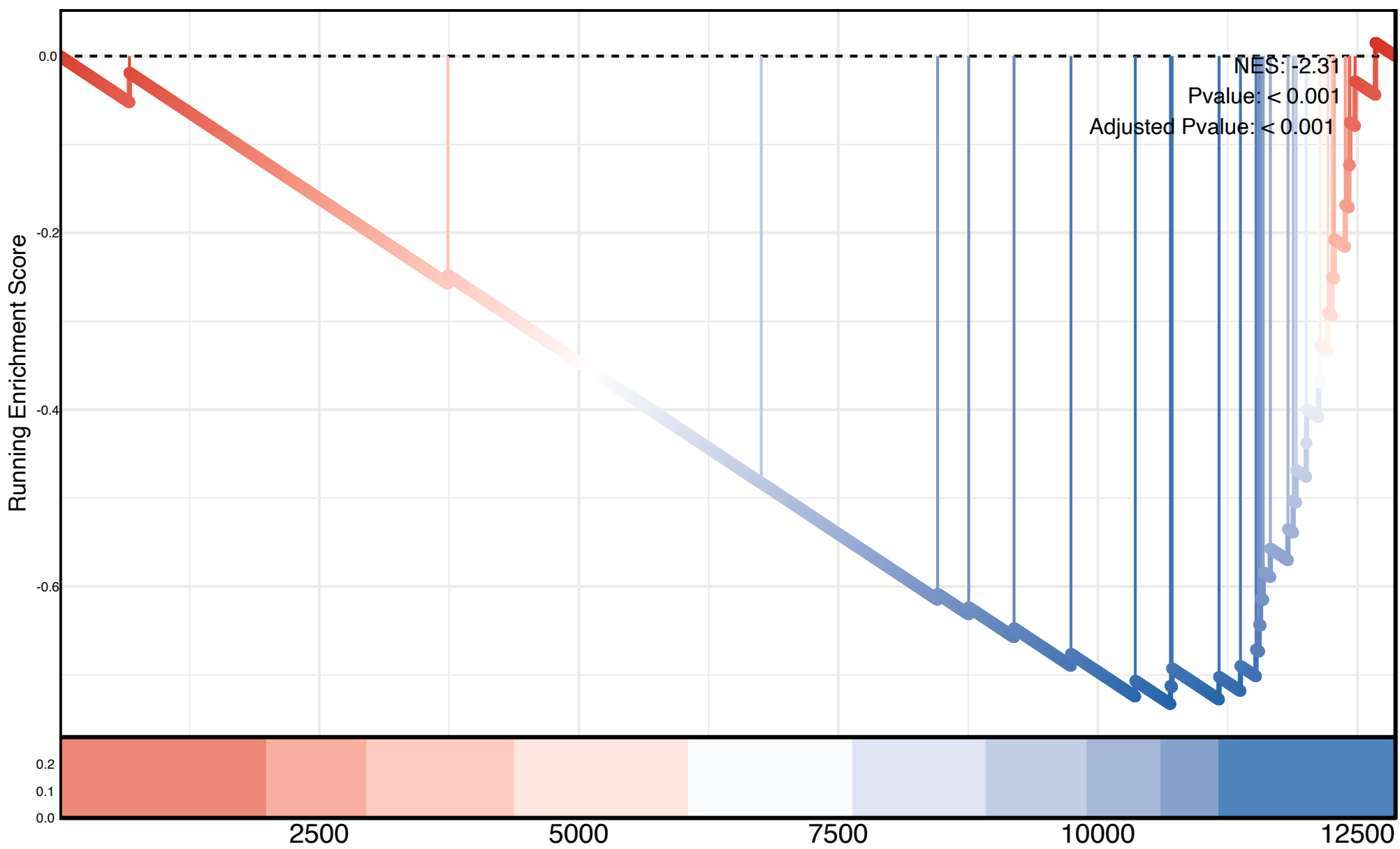
Medicus Reference Homologous Recombination
