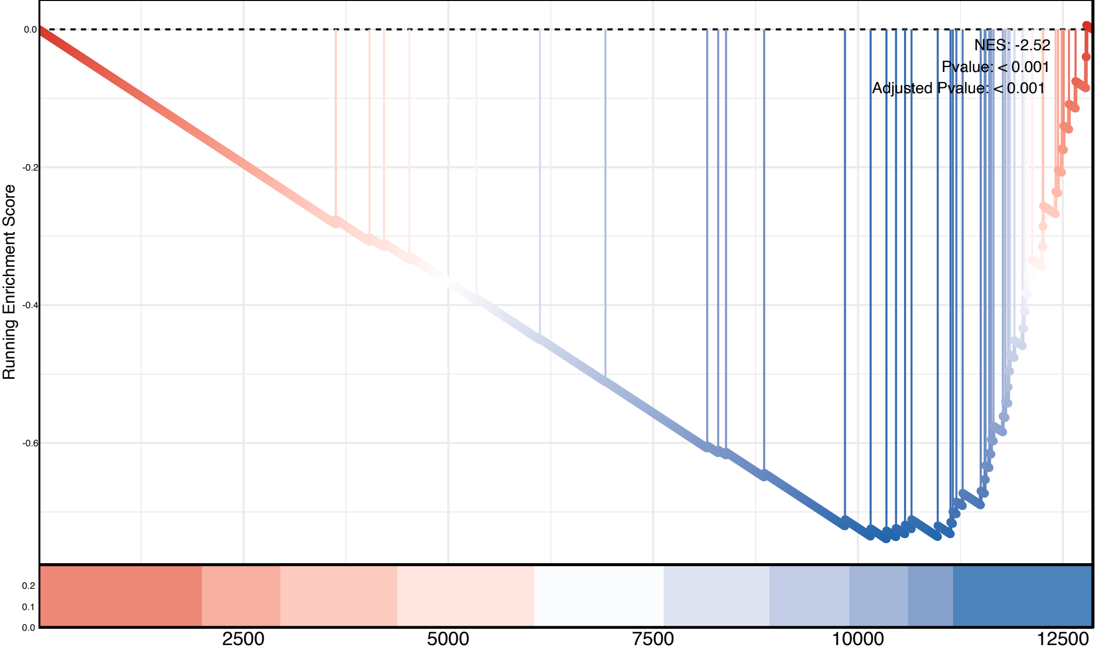
U2 Type Precatalytic Spliceosome
