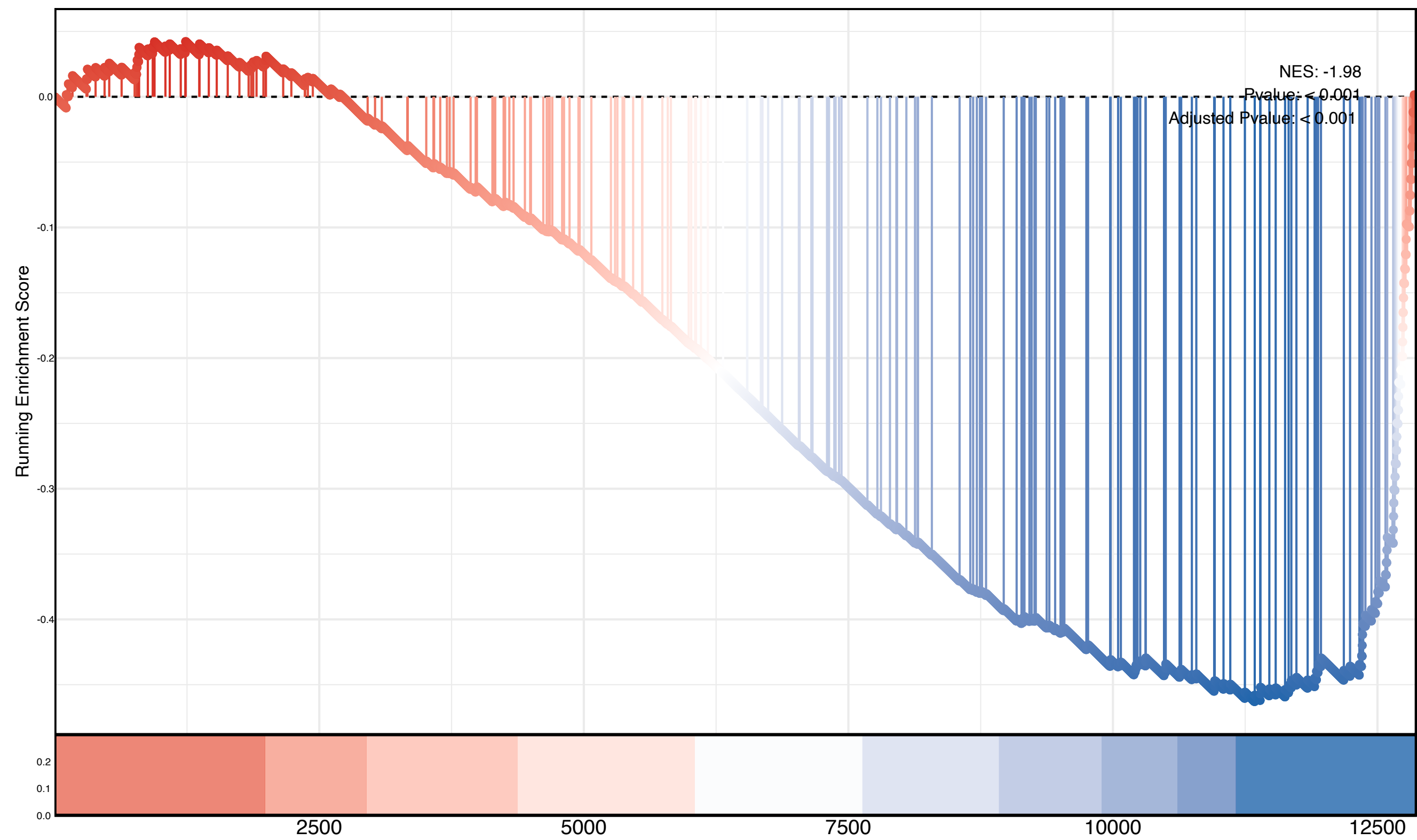
Microtubule Binding
