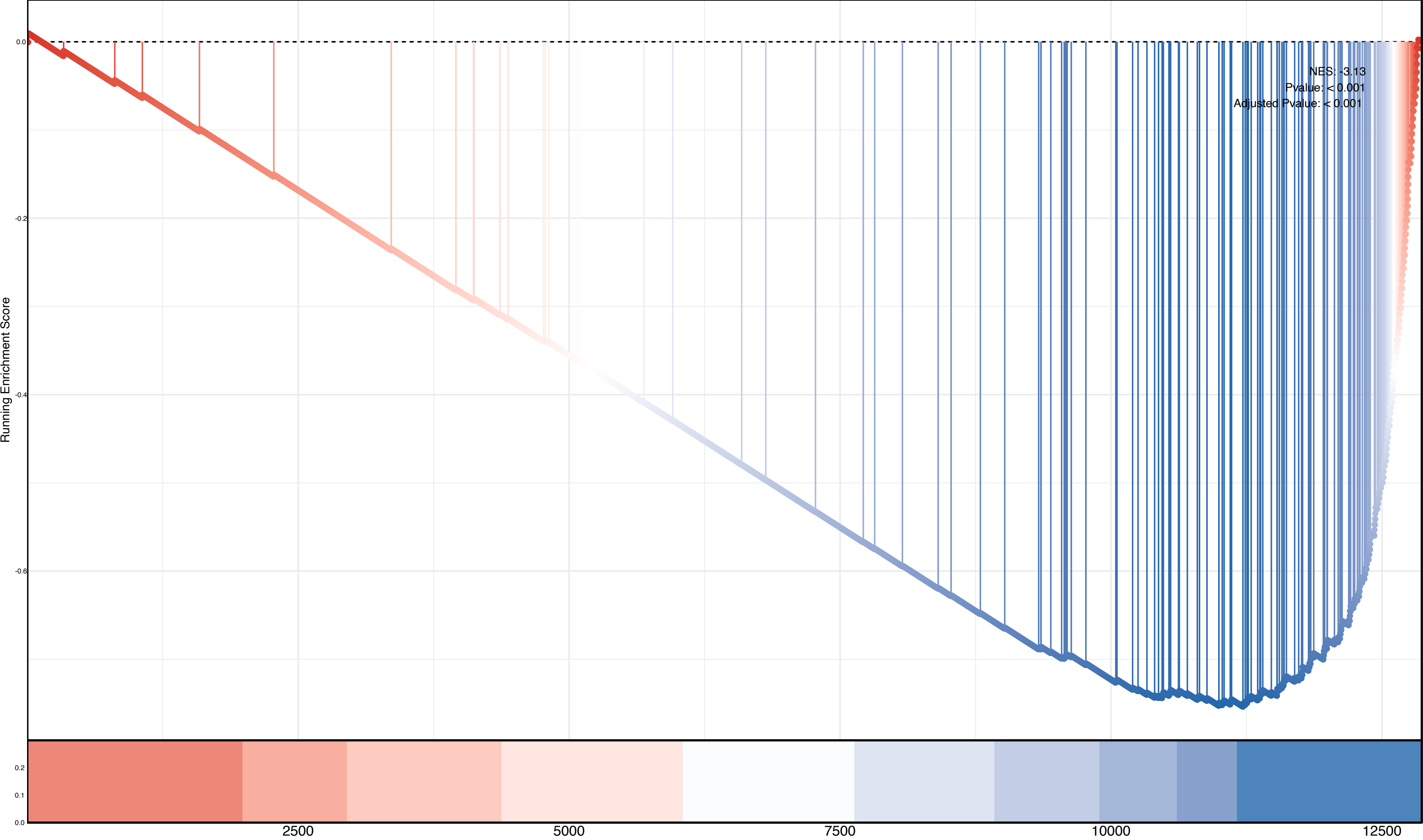
G2m Checkpoint
