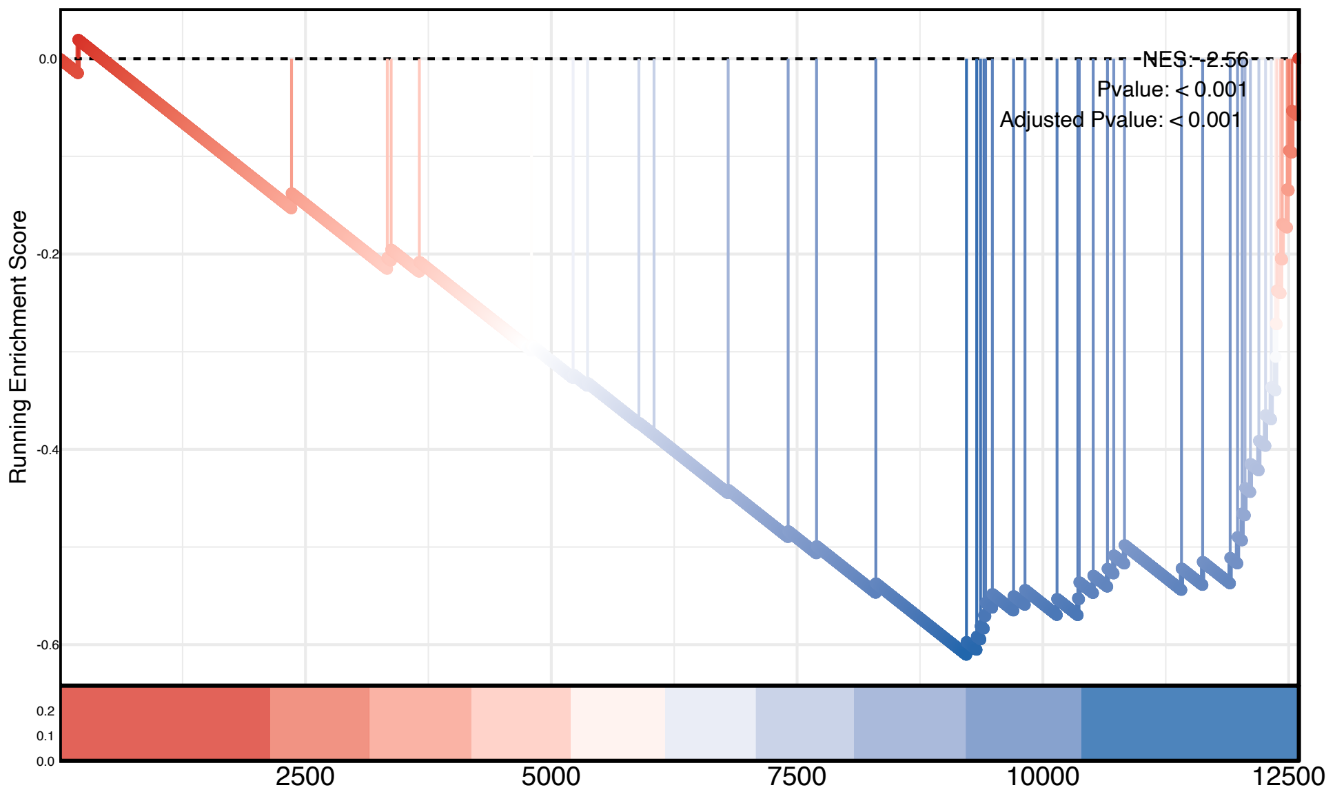
Translation Initiation Factor Activity
