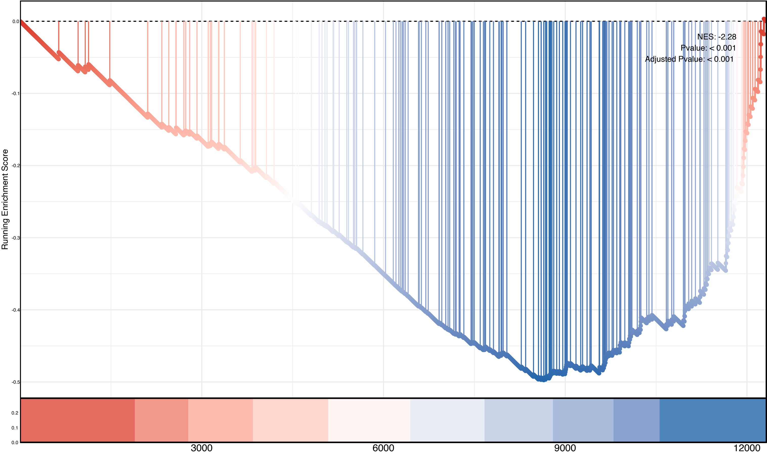
Rrna Processing
